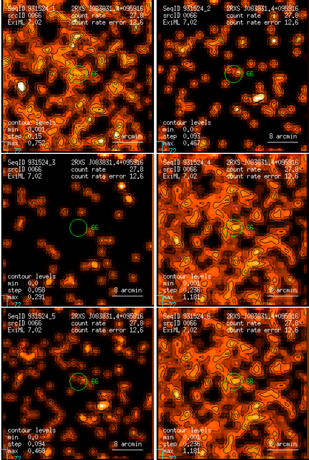
Figure 66: RASS 931524: detection 0066: band rate images, Gaussian filter: (1) PSPC channels 11 – 41, (2) 52 – 90, (3) 91 – 201, (4) 11 – 235, (5) 52 – 201, (6) 11 – 201. Broad band rates in counts/ks. Band rate contour levels in counts/ks/arcmin 2 .
