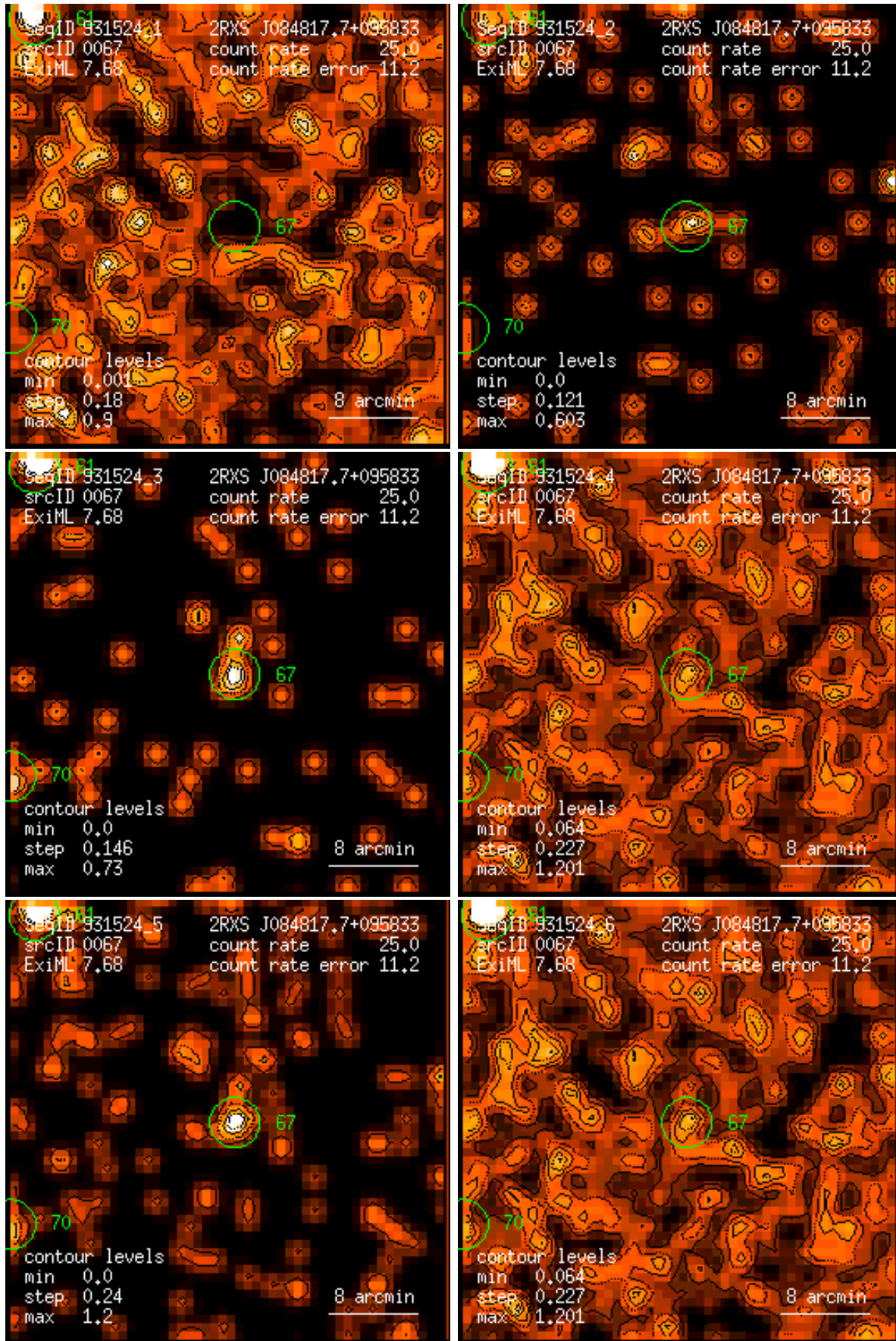
Figure 67: RASS 931524: detection 0067: band rate images, Gaussian filter: (1) PSPC channels 11 – 41, (2) 52 – 90, (3) 91 – 201, (4) 11 – 235, (5) 52 – 201, (6) 11 – 201. Broad band rates in counts/ks. Band rate contour levels in counts/ks/arcmin 2 .
