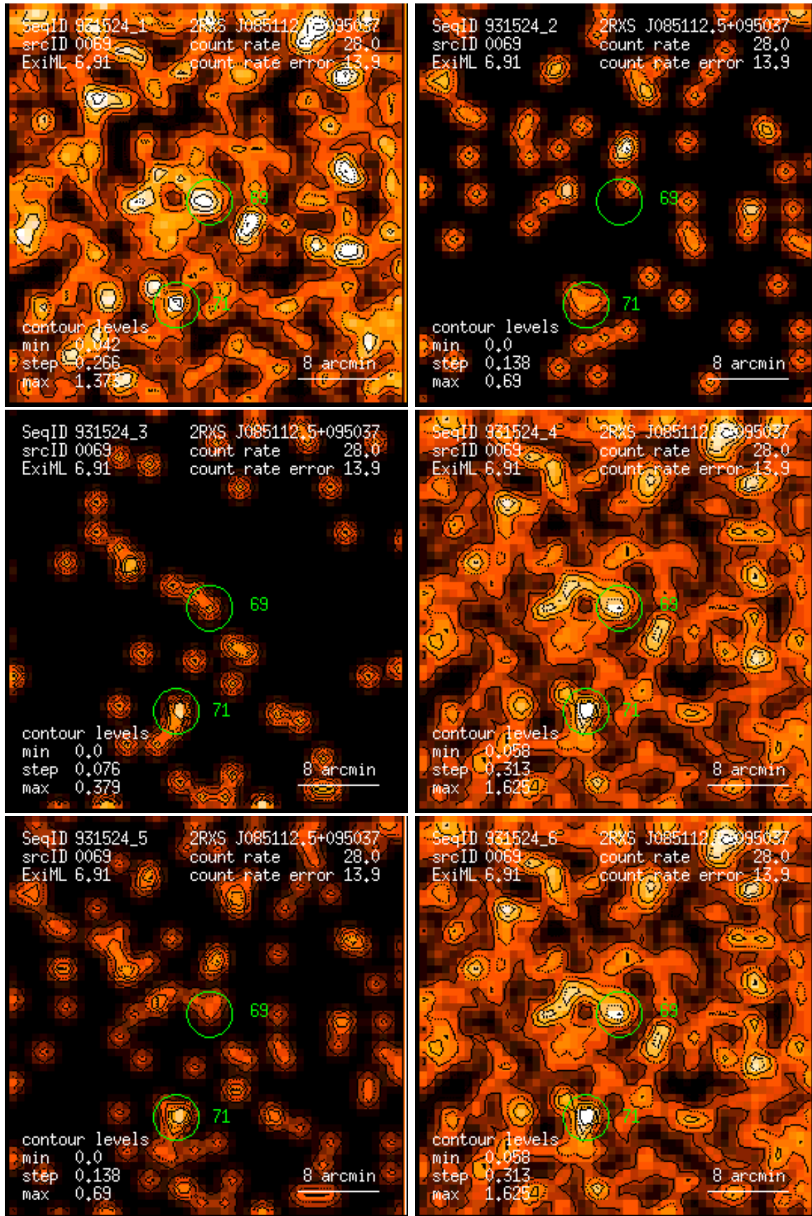
Figure 69: RASS 931524: detection 0069: band rate images, Gaussian filter: (1) PSPC channels 11 – 41, (2) 52 – 90, (3) 91 – 201, (4) 11 – 235, (5) 52 – 201, (6) 11 – 201. Broad band rates in counts/ks. Band rate contour levels in counts/ks/arcmin 2 .
