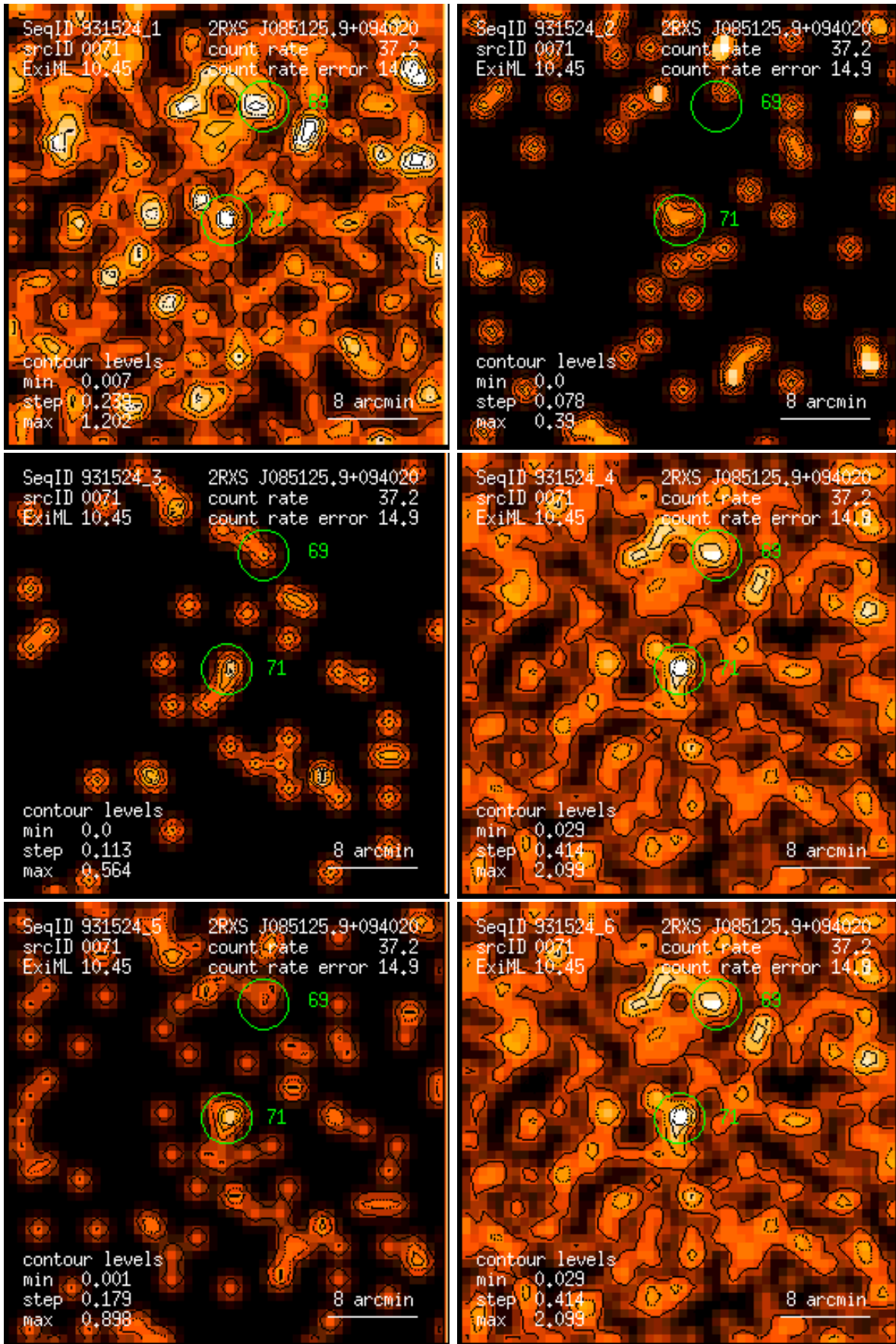
Figure 71: RASS 931524: detection 0071: band rate images, Gaussian filter: (1) PSPC channels 11 – 41, (2) 52 – 90, (3) 91 – 201, (4) 11 – 235, (5) 52 – 201, (6) 11 – 201. Broad band rates in counts/ks. Band rate contour levels in counts/ks/arcmin 2 .
