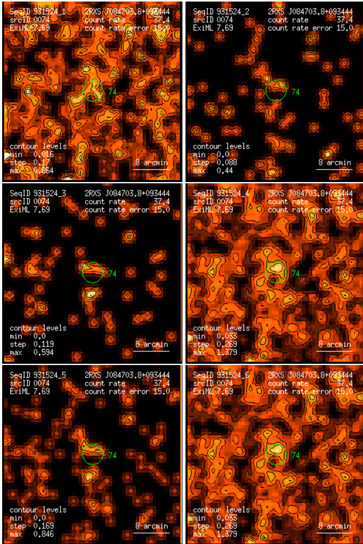
Figure 74: RASS 931524: detection 0074: band rate images, Gaussian filter: (1) PSPC channels 11 – 41, (2) 52 – 90, (3) 91 – 201, (4) 11 – 235, (5) 52 – 201, (6) 11 – 201. Broad band rates in counts/ks. Band rate contour levels in counts/ks/arcmin 2 .
