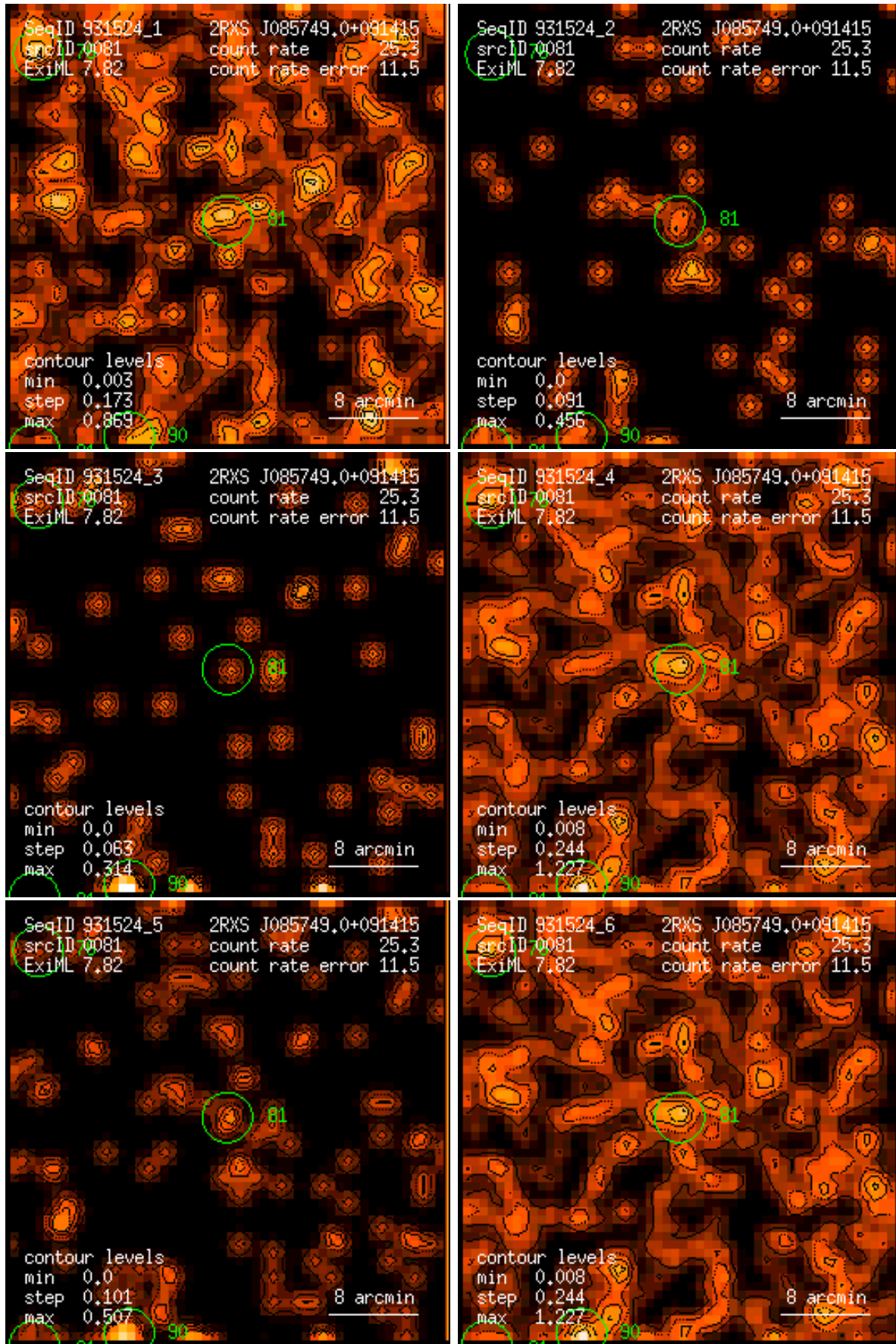
Figure 81: RASS 931524: detection 0081: band rate images, Gaussian filter: (1) PSPC channels 11 – 41, (2) 52 – 90, (3) 91 – 201, (4) 11 – 235, (5) 52 – 201, (6) 11 – 201. Broad band rates in counts/ks. Band rate contour levels in counts/ks/arcmin 2 .
