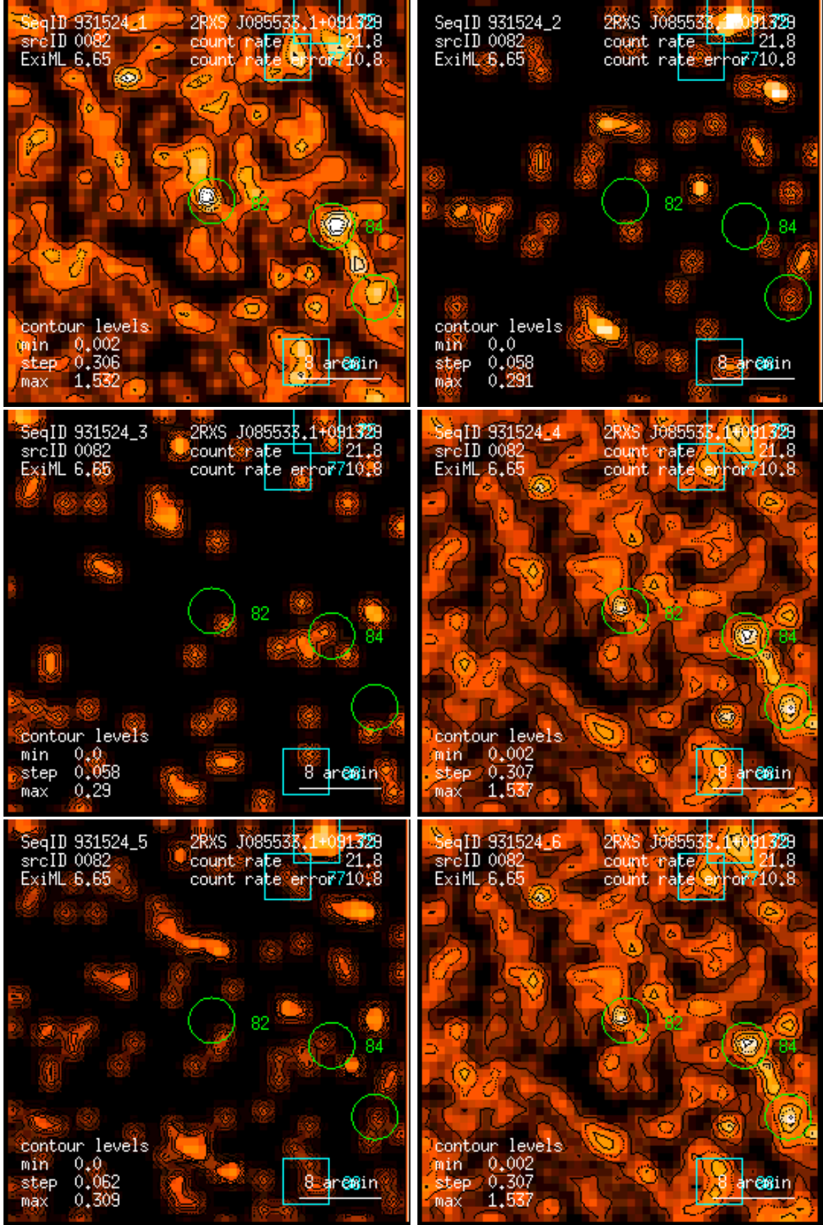
Figure 82: RASS 931524: detection 0082: band rate images, Gaussian filter: (1) PSPC channels 11 – 41, (2) 52 – 90, (3) 91 – 201, (4) 11 – 235, (5) 52 – 201, (6) 11 – 201. Broad band rates in counts/ks. Band rate contour levels in counts/ks/arcmin 2 .
