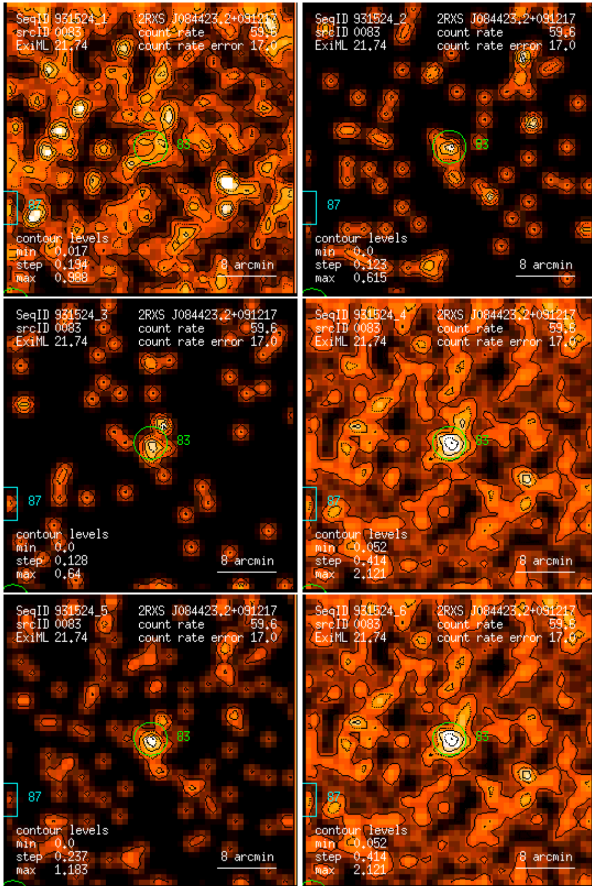
Figure 83: RASS 931524: detection 0083: band rate images, Gaussian filter: (1) PSPC channels 11 – 41, (2) 52 – 90, (3) 91 – 201, (4) 11 – 235, (5) 52 – 201, (6) 11 – 201. Broad band rates in counts/ks. Band rate contour levels in counts/ks/arcmin 2 .
