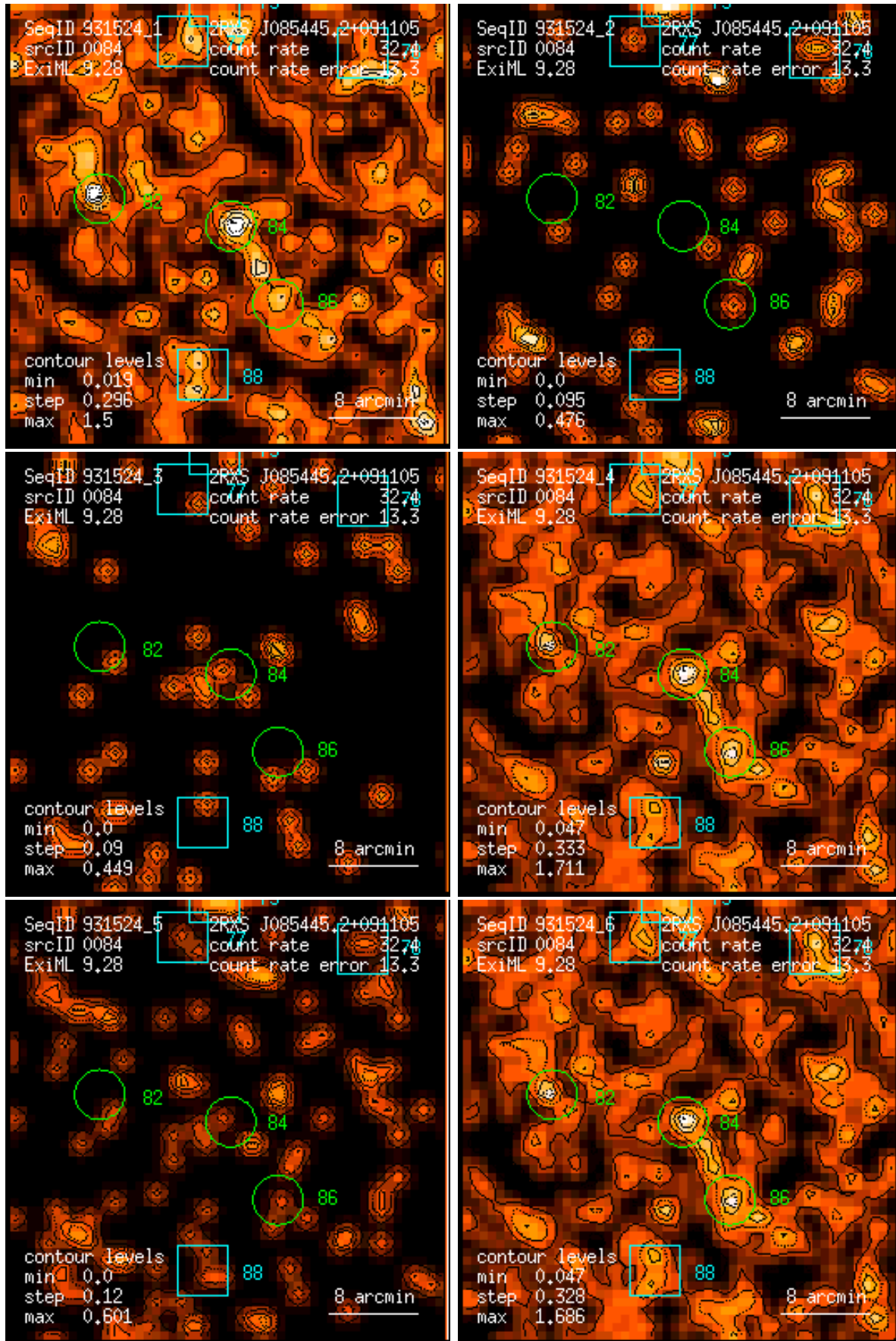
Figure 84: RASS 931524: detection 0084: band rate images, Gaussian filter: (1) PSPC channels 11 – 41, (2) 52 – 90, (3) 91 – 201, (4) 11 – 235, (5) 52 – 201, (6) 11 – 201. Broad band rates in counts/ks. Band rate contour levels in counts/ks/arcmin 2 .
