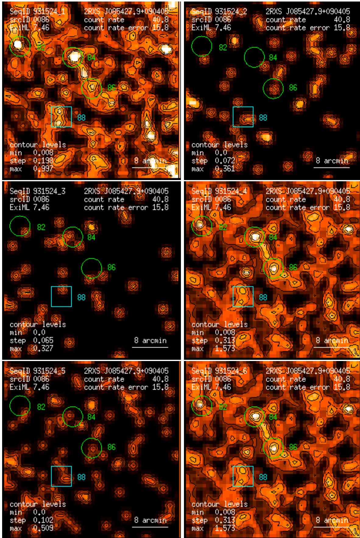
Figure 86: RASS 931524: detection 0086: band rate images, Gaussian filter: (1) PSPC channels 11 – 41, (2) 52 – 90, (3) 91 – 201, (4) 11 – 235, (5) 52 – 201, (6) 11 – 201. Broad band rates in counts/ks. Band rate contour levels in counts/ks/arcmin 2 .
