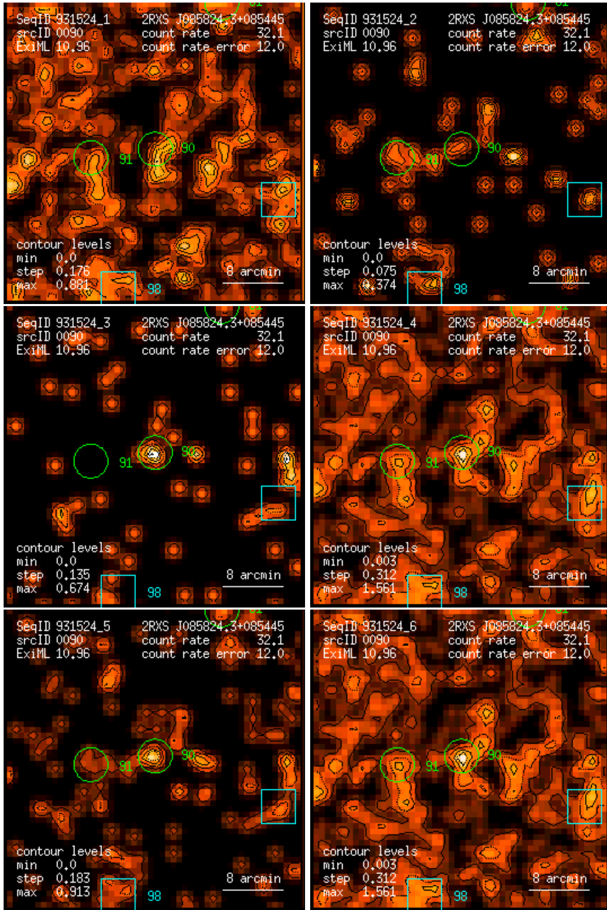
Figure 90: RASS 931524: detection 0090: band rate images, Gaussian filter: (1) PSPC channels 11 – 41, (2) 52 – 90, (3) 91 – 201, (4) 11 – 235, (5) 52 – 201, (6) 11 – 201. Broad band rates in counts/ks. Band rate contour levels in counts/ks/arcmin 2 .
