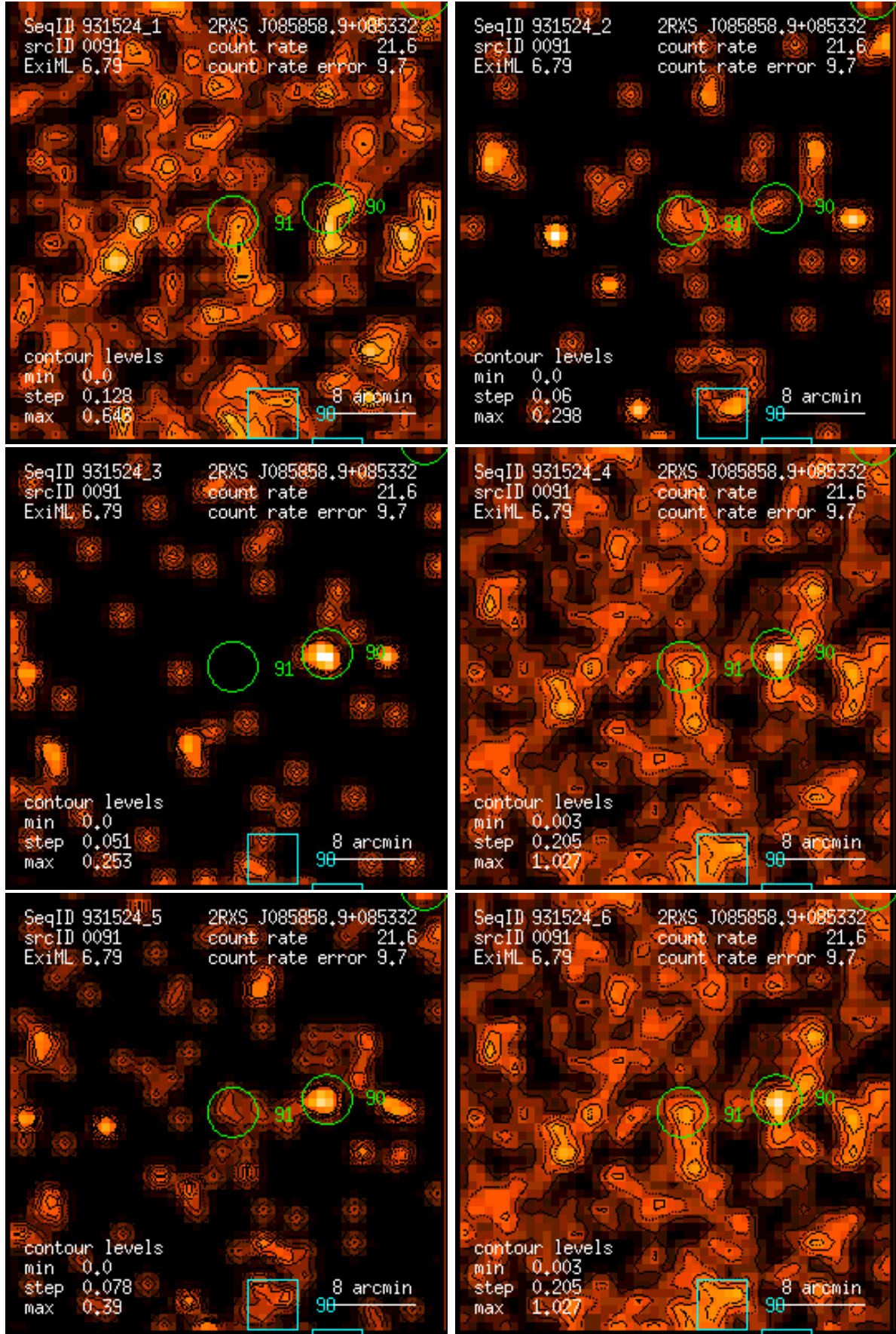
Figure 91: RASS 931524: detection 0091: band rate images, Gaussian filter: (1) PSPC channels 11 – 41, (2) 52 – 90, (3) 91 – 201, (4) 11 – 235, (5) 52 – 201, (6) 11 – 201. Broad band rates in counts/ks. Band rate contour levels in counts/ks/arcmin 2 .
