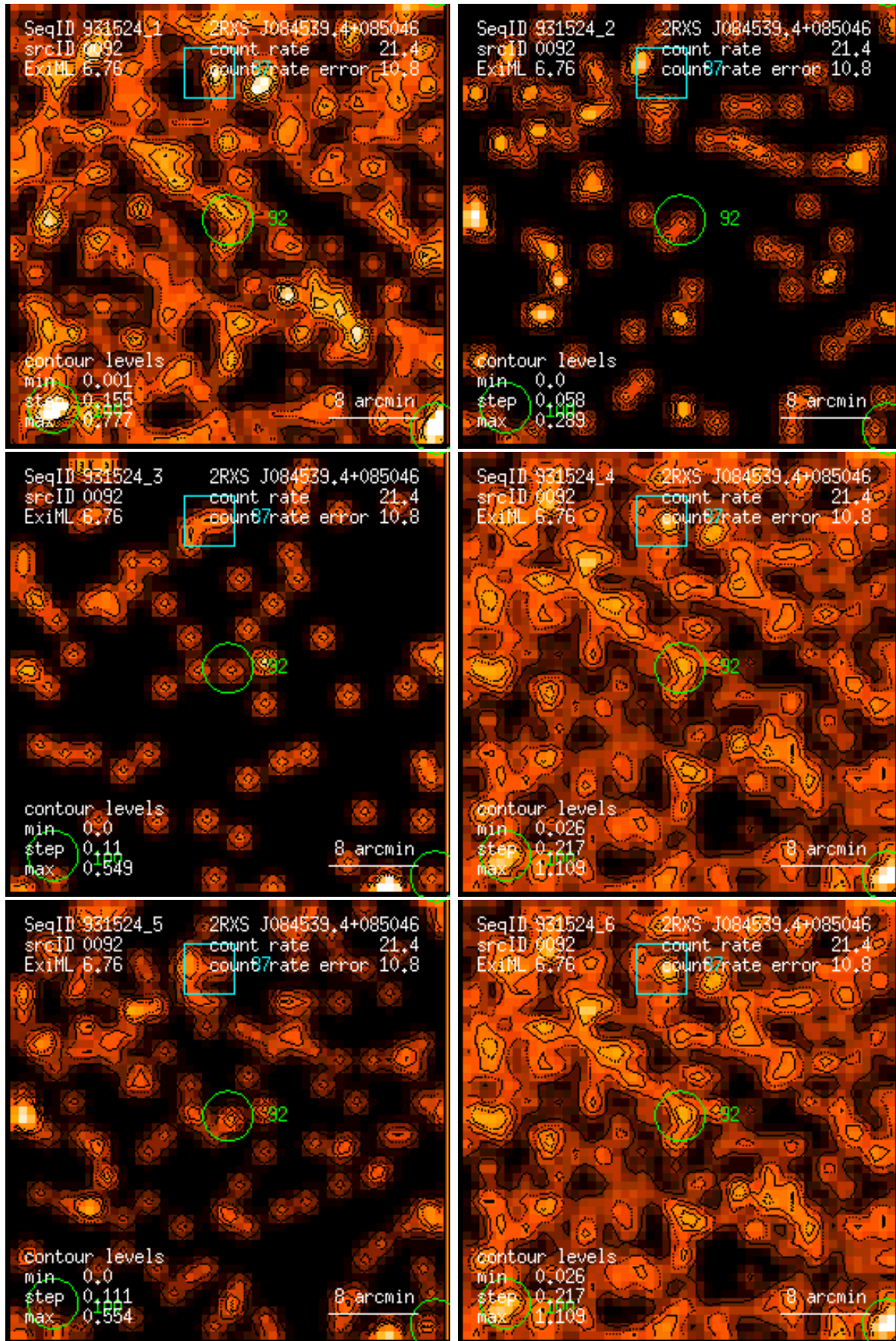
Figure 92: RASS 931524: detection 0092: band rate images, Gaussian filter: (1) PSPC channels 11 – 41, (2) 52 – 90, (3) 91 – 201, (4) 11 – 235, (5) 52 – 201, (6) 11 – 201. Broad band rates in counts/ks. Band rate contour levels in counts/ks/arcmin 2 .
