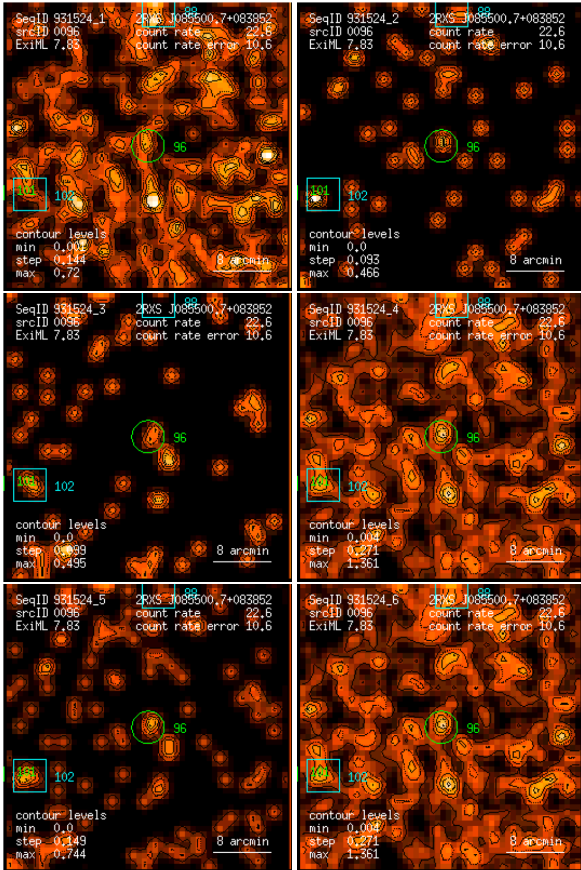
Figure 96: RASS 931524: detection 0096: band rate images, Gaussian filter: (1) PSPC channels 11 – 41, (2) 52 – 90, (3) 91 – 201, (4) 11 – 235, (5) 52 – 201, (6) 11 – 201. Broad band rates in counts/ks. Band rate contour levels in counts/ks/arcmin 2 .
