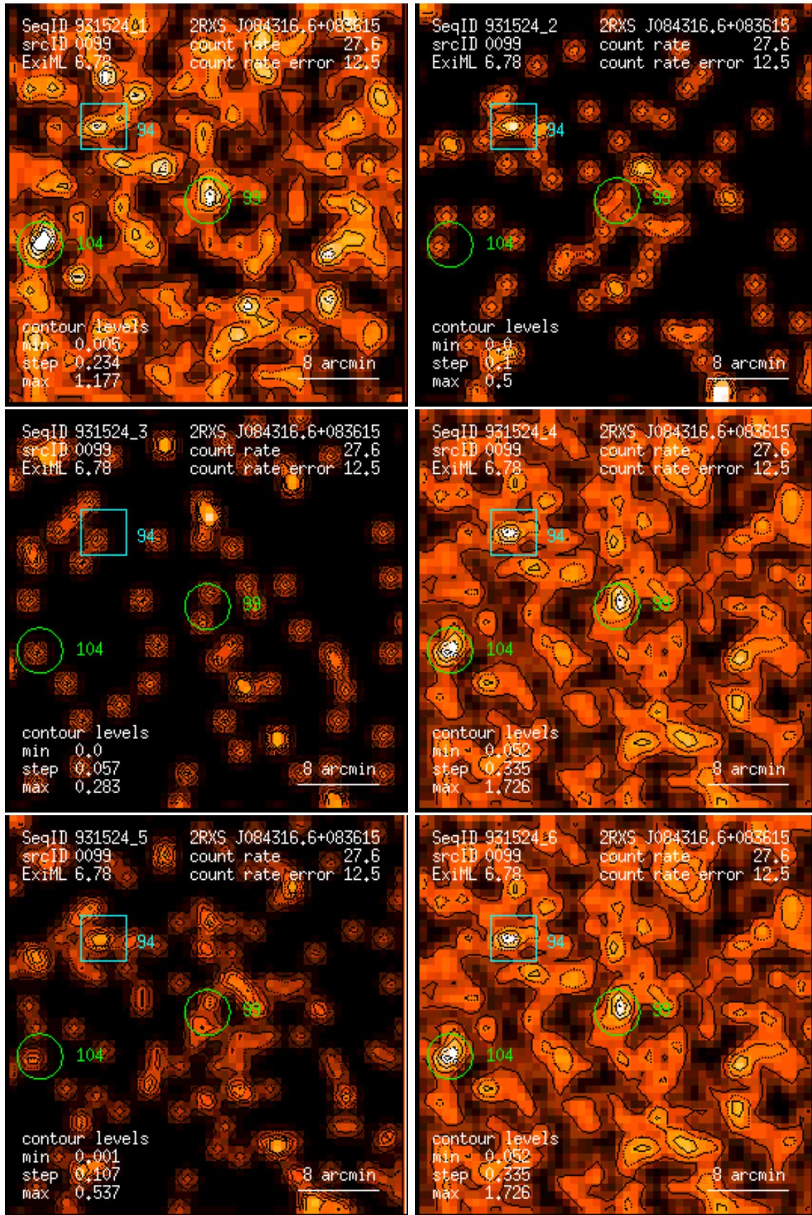
Figure 99: RASS 931524: detection 0099: band rate images, Gaussian filter: (1) PSPC channels 11 – 41, (2) 52 – 90, (3) 91 – 201, (4) 11 – 235, (5) 52 – 201, (6) 11 – 201. Broad band rates in counts/ks. Band rate contour levels in counts/ks/arcmin 2 .
