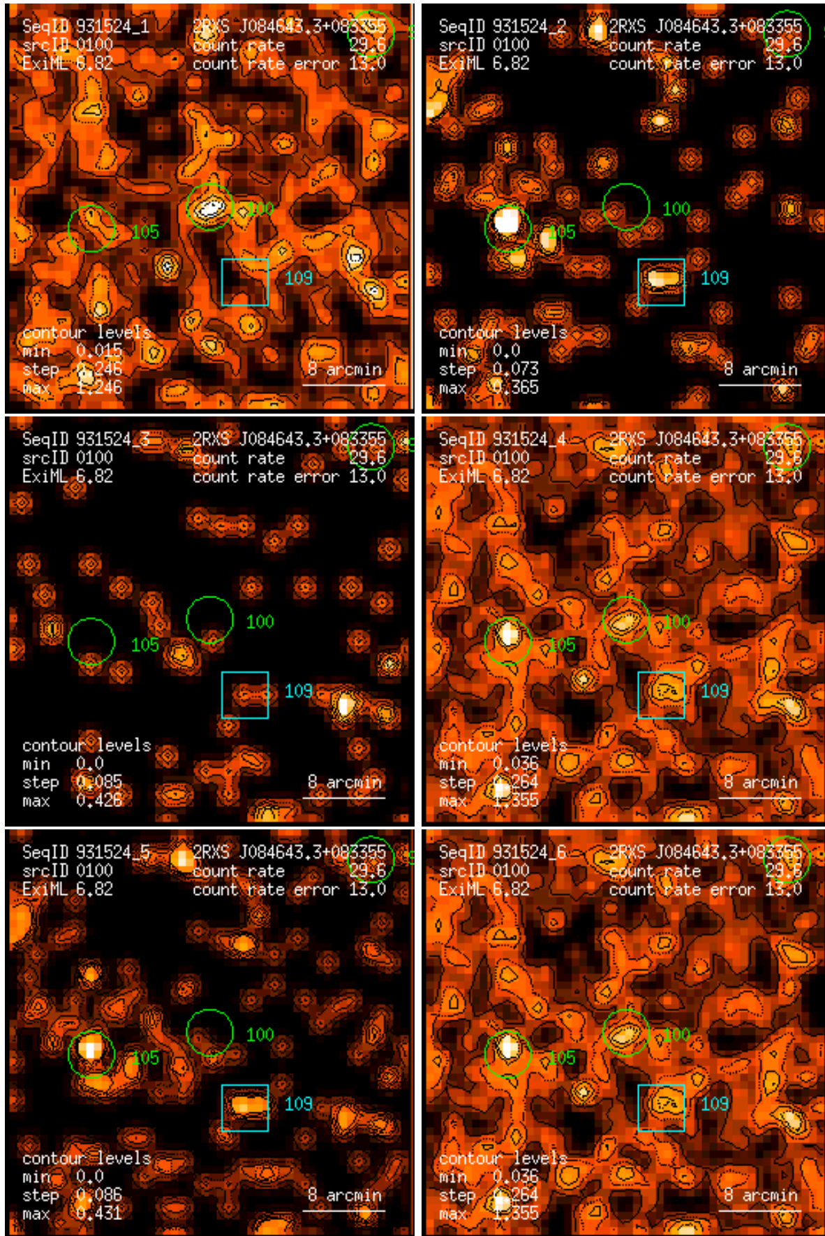
Figure 100: RASS 931524: detection 0100: band rate images, Gaussian filter: (1) PSPC channels 11 – 41, (2) 52 – 90, (3) 91 – 201, (4) 11 – 235, (5) 52 – 201, (6) 11 – 201. Broad band rates in counts/ks. Band rate contour levels in counts/ks/arcmin 2 .
