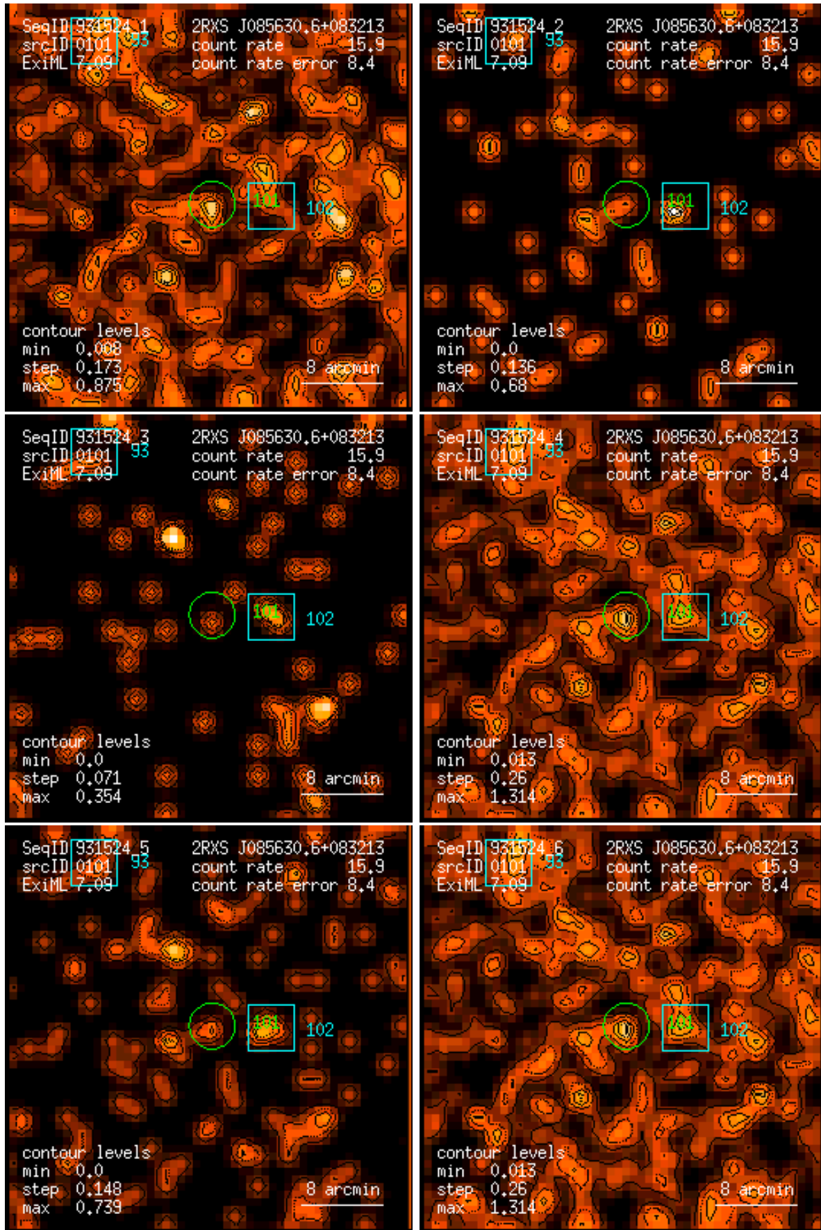
Figure 101: RASS 931524: detection 0101: band rate images, Gaussian filter: (1) PSPC channels 11 – 41, (2) 52 – 90, (3) 91 – 201, (4) 11 – 235, (5) 52 – 201, (6) 11 – 201. Broad band rates in counts/ks. Band rate contour levels in counts/ks/arcmin 2 .
