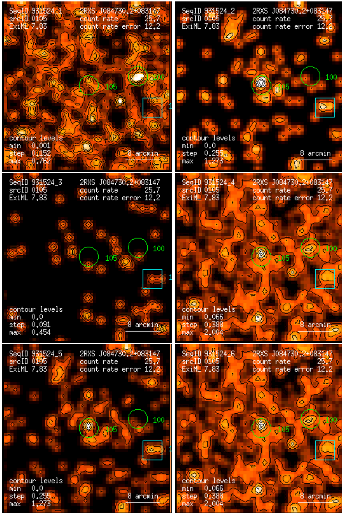
Figure 105: RASS 931524: detection 0105: band rate images, Gaussian filter: (1) PSPC channels 11 – 41, (2) 52 – 90, (3) 91 – 201, (4) 11 – 235, (5) 52 – 201, (6) 11 – 201. Broad band rates in counts/ks. Band rate contour levels in counts/ks/arcmin 2 .
