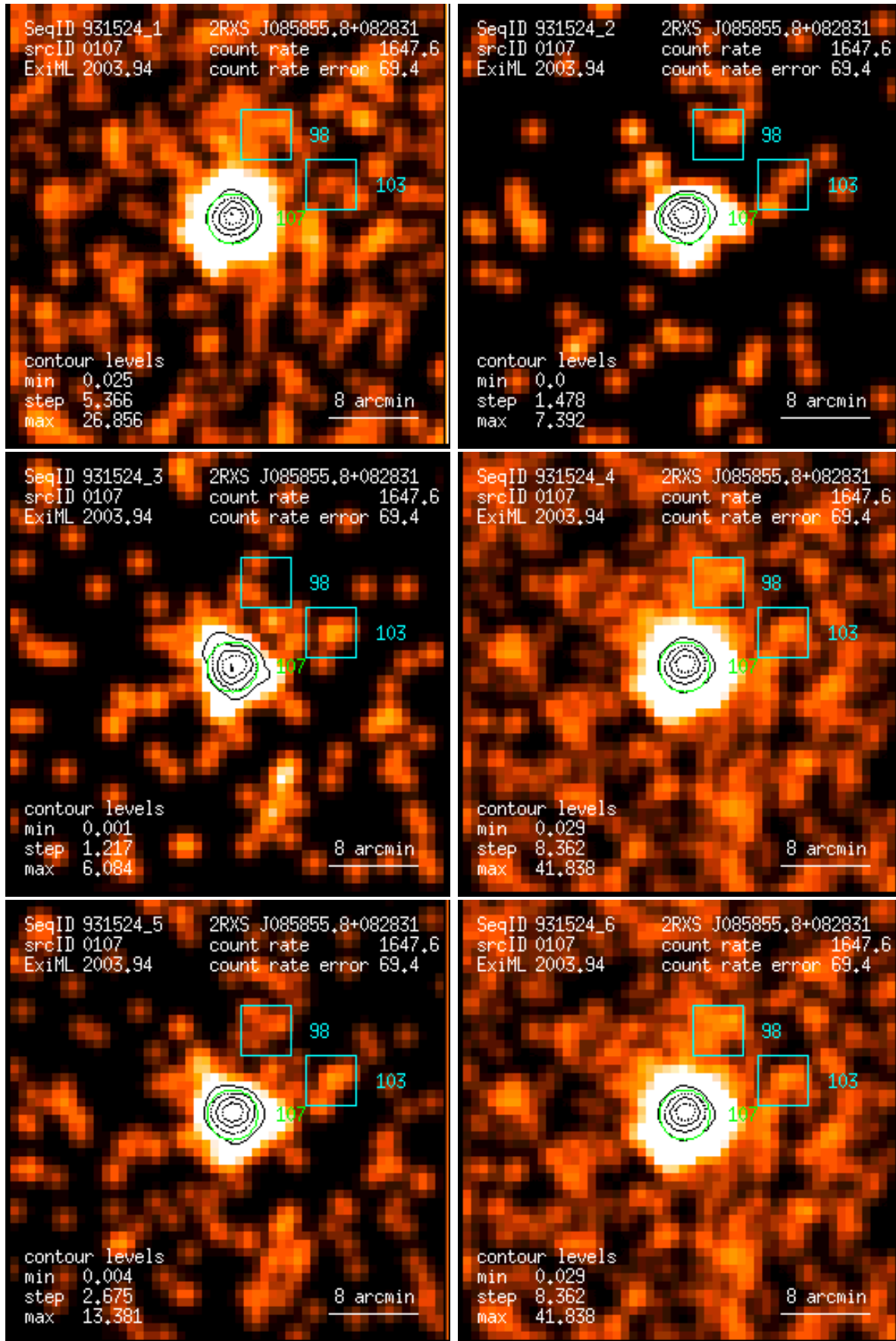
Figure 107: RASS 931524: detection 0107: band rate images, Gaussian filter: (1) PSPC channels 11 – 41, (2) 52 – 90, (3) 91 – 201, (4) 11 – 235, (5) 52 – 201, (6) 11 – 201. Broad band rates in counts/ks. Band rate contour levels in counts/ks/arcmin 2 .
