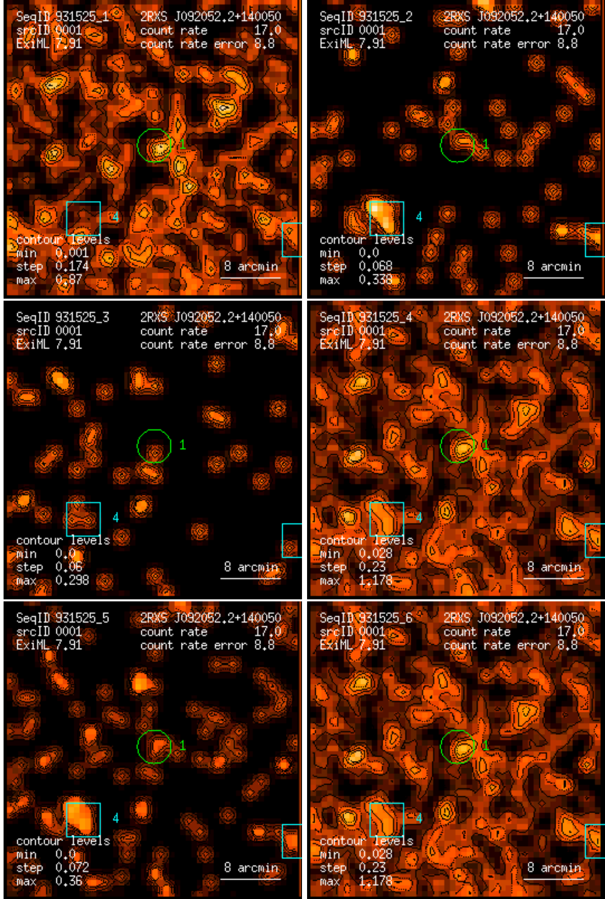
Figure 1: RASS 931525: detection 0001: band rate images, Gaussian filter: (1) PSPC channels 11 – 41, (2) 52 – 90, (3) 91 – 201, (4) 11 – 235, (5) 52 – 201, (6) 11 – 201. Broad band rates in counts/ks. Band rate contour levels in counts/ks/arcmin 2 .
