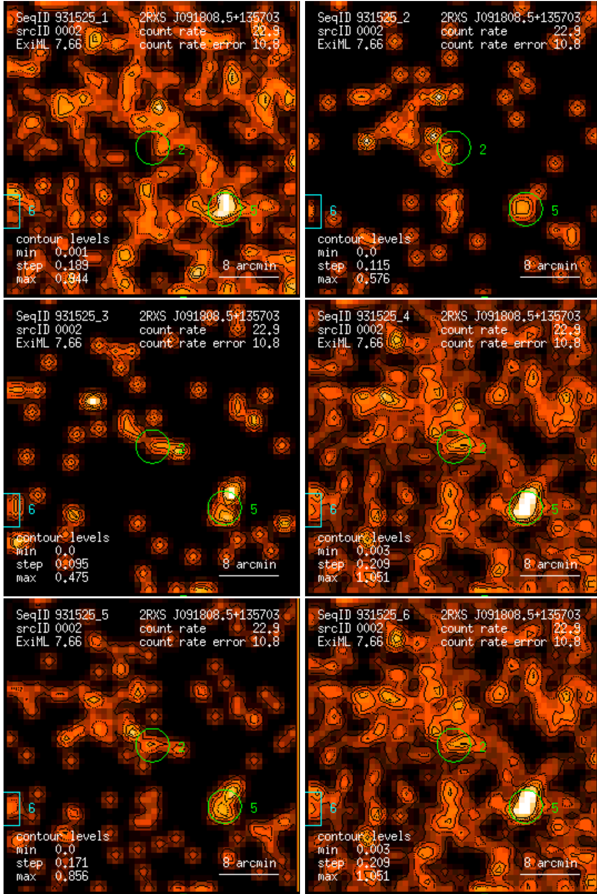
Figure 2: RASS 931525: detection 0002: band rate images, Gaussian filter: (1) PSPC channels 11 – 41, (2) 52 – 90, (3) 91 – 201, (4) 11 – 235, (5) 52 – 201, (6) 11 – 201. Broad band rates in counts/ks. Band rate contour levels in counts/ks/arcmin 2 .
