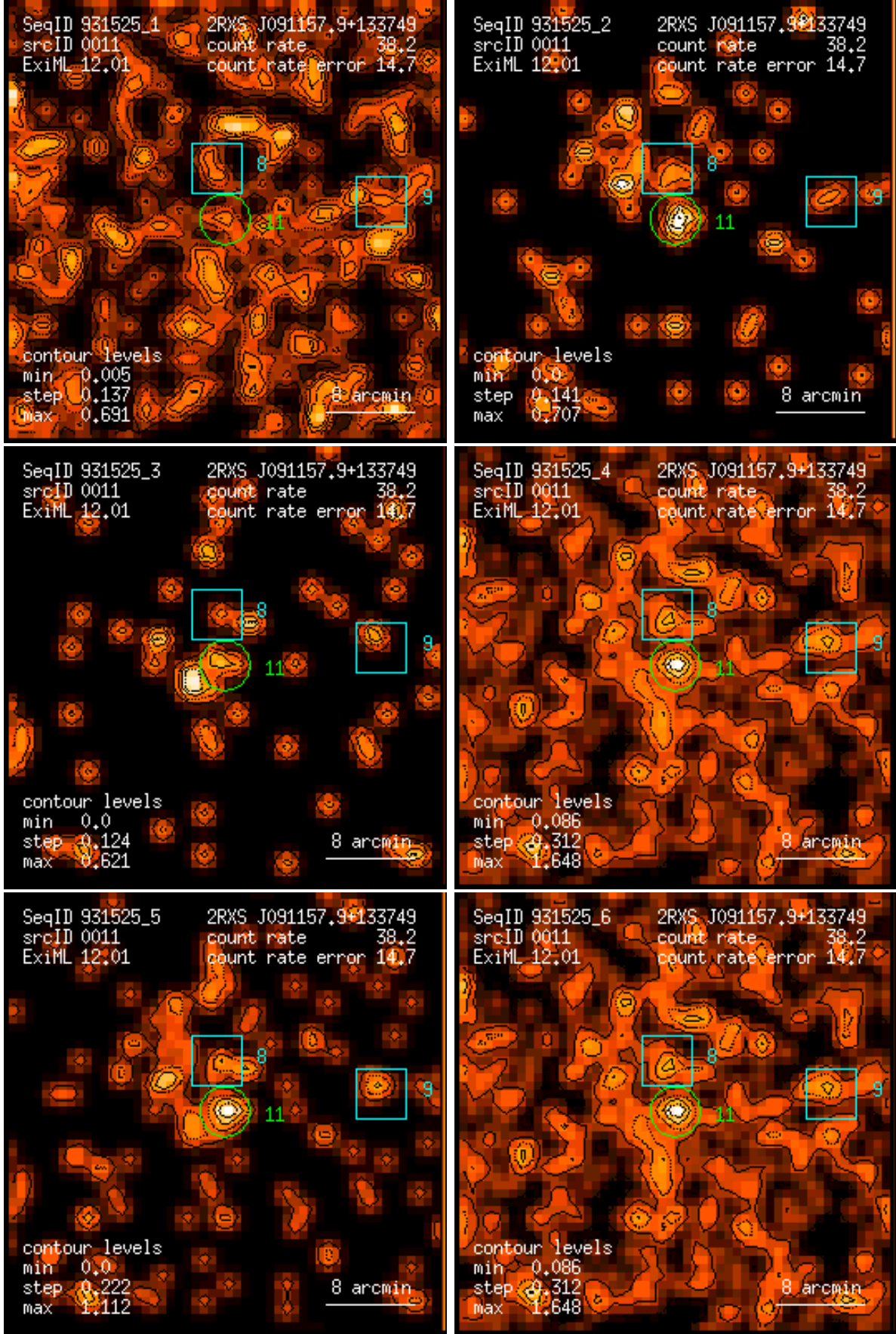
Figure 11: RASS 931525: detection 0011: band rate images, Gaussian filter: (1) PSPC channels 11 – 41, (2) 52 – 90, (3) 91 – 201, (4) 11 – 235, (5) 52 – 201, (6) 11 – 201. Broad band rates in counts/ks. Band rate contour levels in counts/ks/arcmin 2 .
