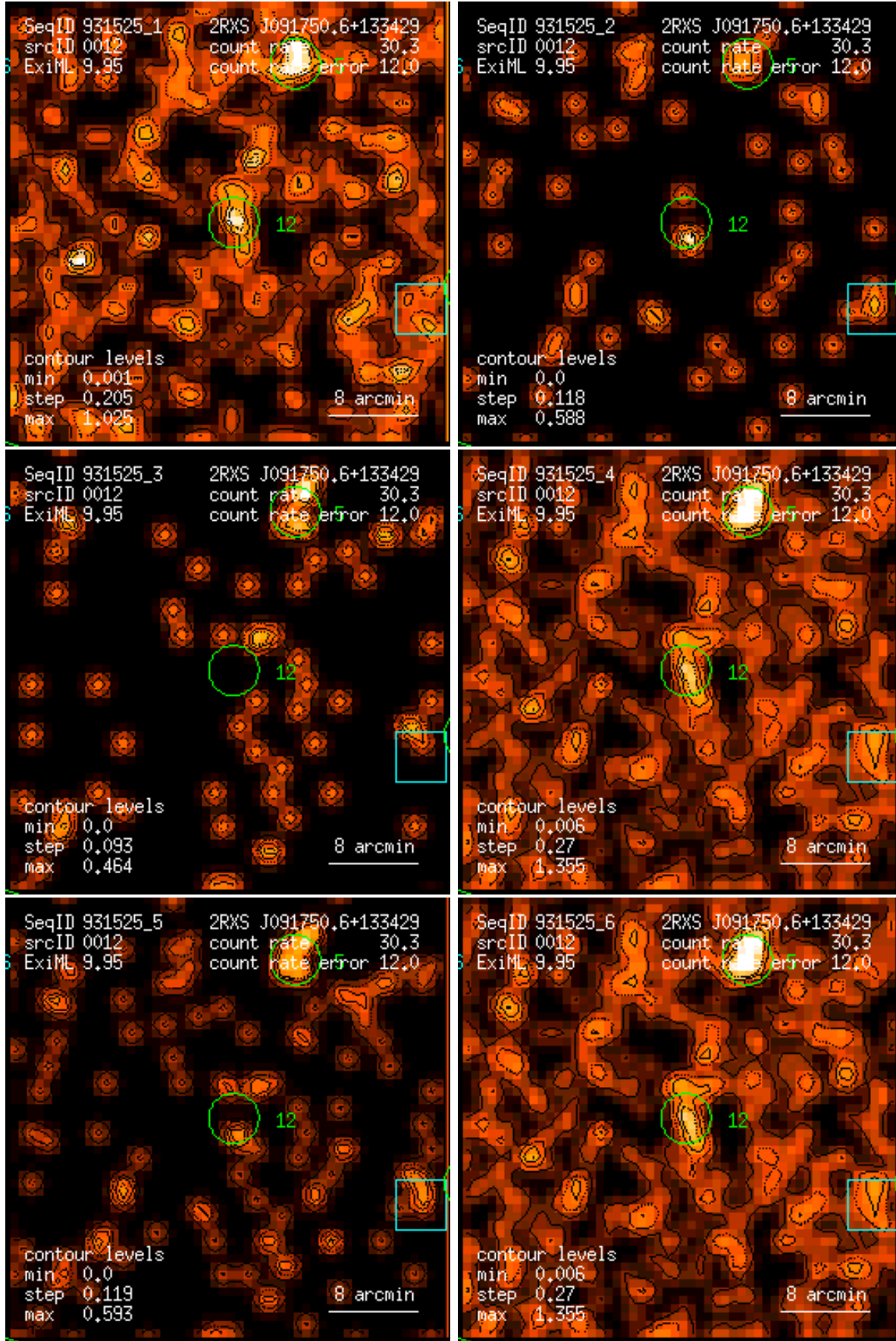
Figure 12: RASS 931525: detection 0012: band rate images, Gaussian filter: (1) PSPC channels 11 – 41, (2) 52 – 90, (3) 91 – 201, (4) 11 – 235, (5) 52 – 201, (6) 11 – 201. Broad band rates in counts/ks. Band rate contour levels in counts/ks/arcmin 2 .
