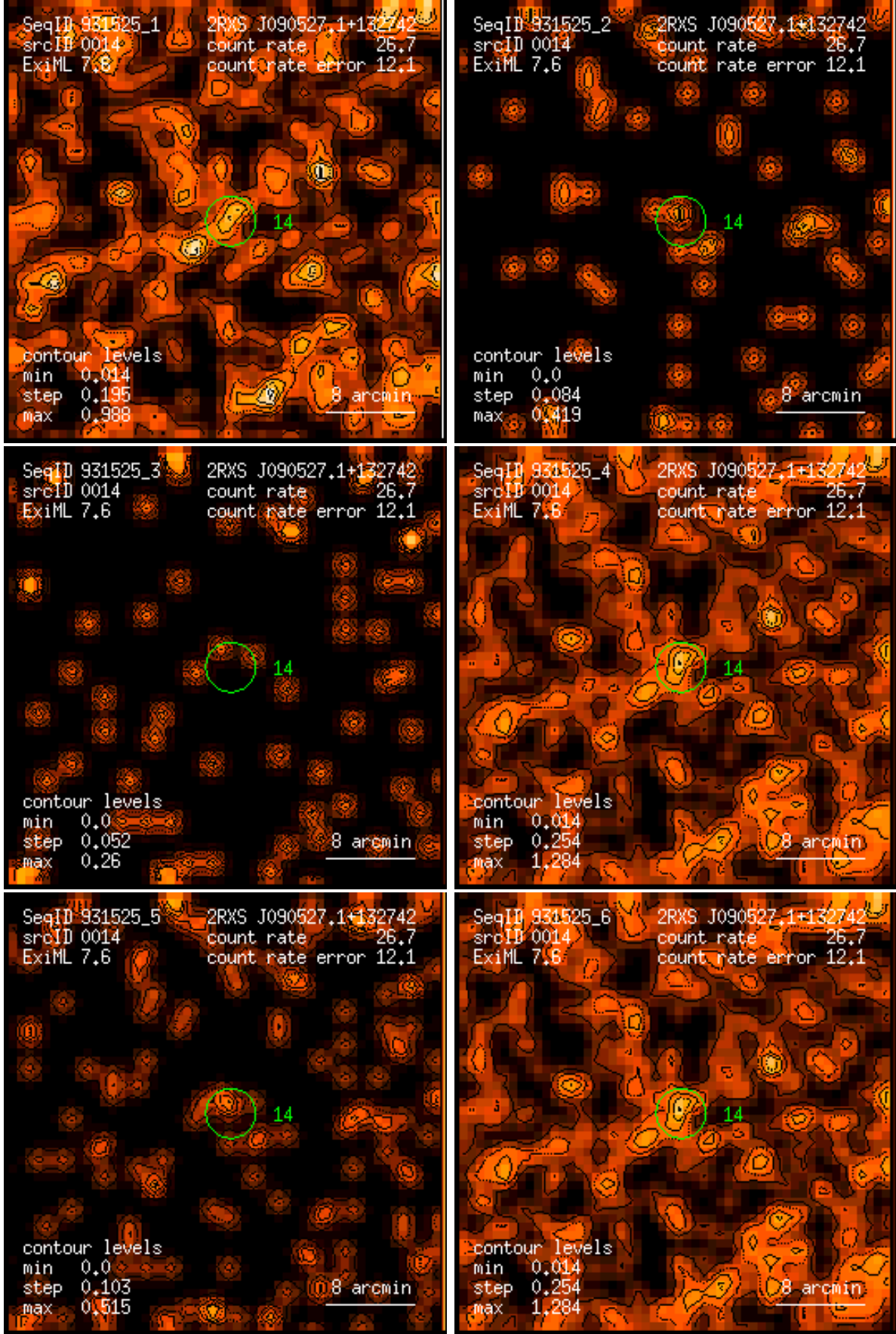
Figure 14: RASS 931525: detection 0014: band rate images, Gaussian filter: (1) PSPC channels 11 – 41, (2) 52 – 90, (3) 91 – 201, (4) 11 – 235, (5) 52 – 201, (6) 11 – 201. Broad band rates in counts/ks. Band rate contour levels in counts/ks/arcmin 2 .
