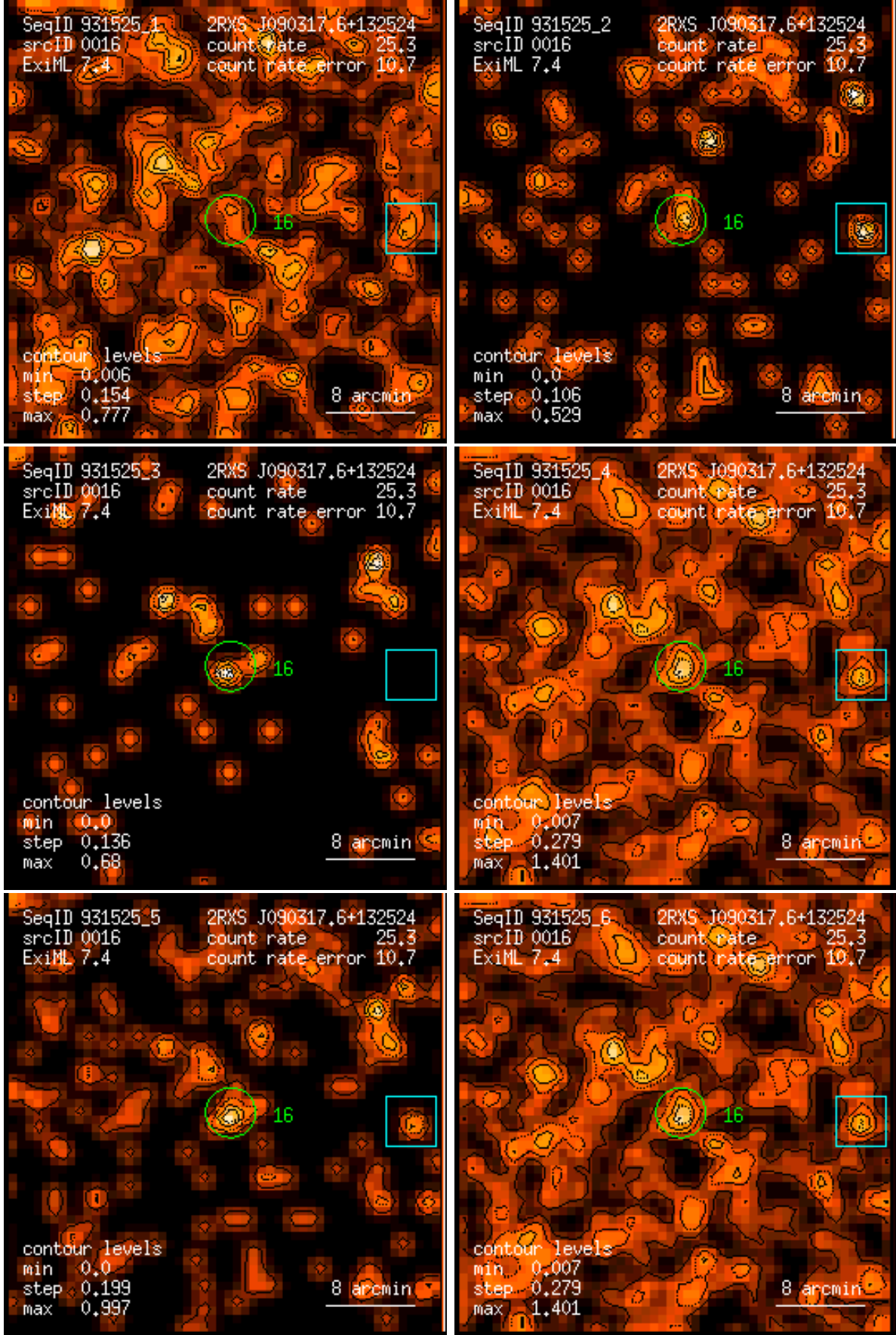
Figure 16: RASS 931525: detection 0016: band rate images, Gaussian filter: (1) PSPC channels 11 – 41, (2) 52 – 90, (3) 91 – 201, (4) 11 – 235, (5) 52 – 201, (6) 11 – 201. Broad band rates in counts/ks. Band rate contour levels in counts/ks/arcmin 2 .
