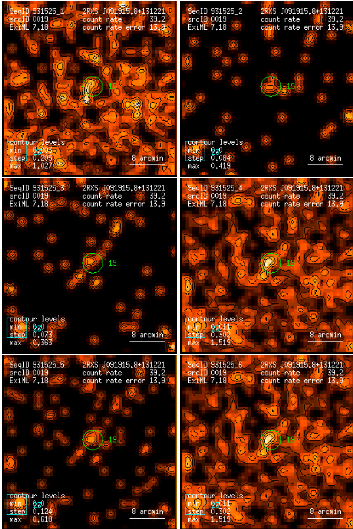
Figure 19: RASS 931525: detection 0019: band rate images, Gaussian filter: (1) PSPC channels 11 – 41, (2) 52 – 90, (3) 91 – 201, (4) 11 – 235, (5) 52 – 201, (6) 11 – 201. Broad band rates in counts/ks. Band rate contour levels in counts/ks/arcmin 2 .
