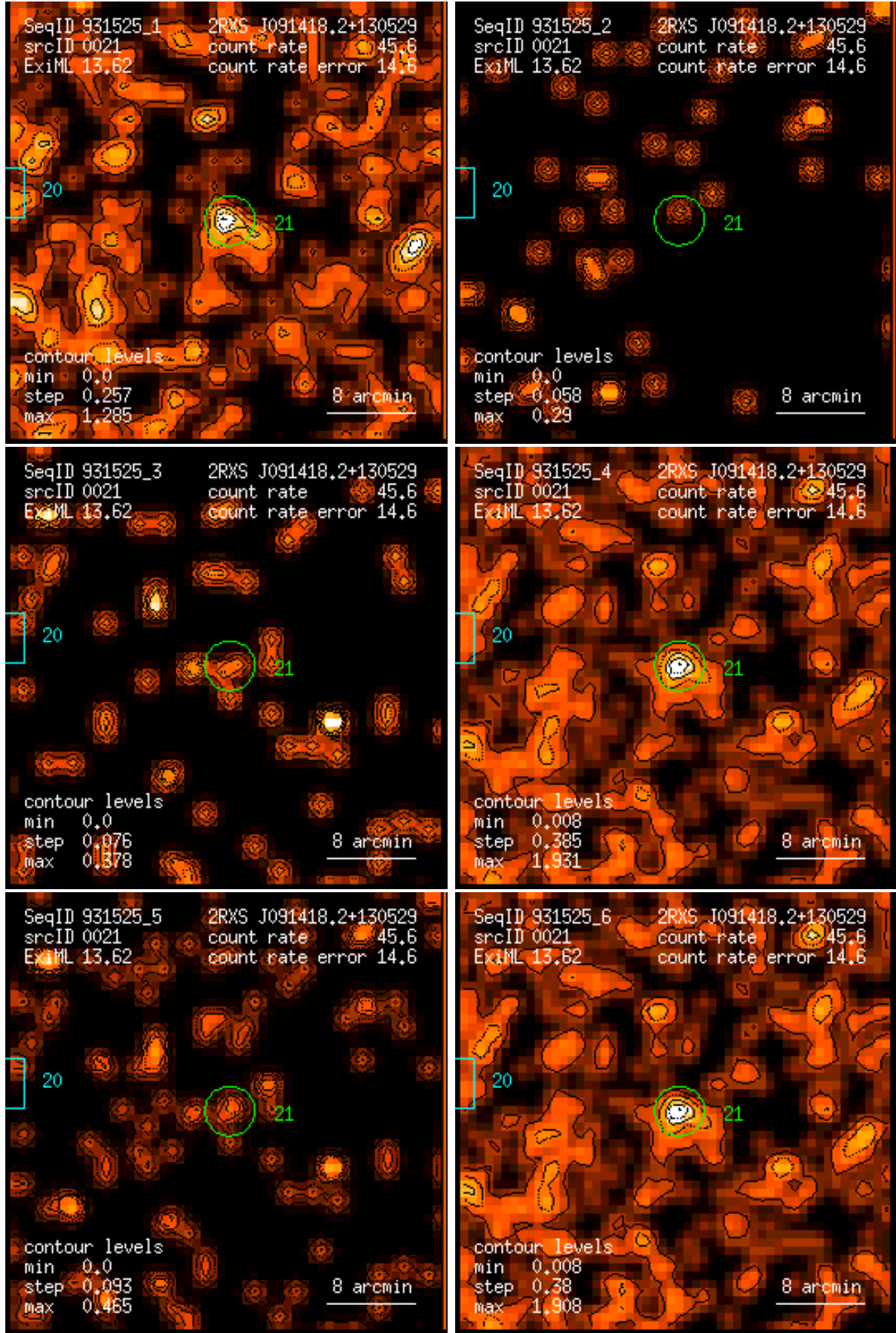
Figure 21: RASS 931525: detection 0021: band rate images, Gaussian filter: (1) PSPC channels 11 – 41, (2) 52 – 90, (3) 91 – 201, (4) 11 – 235, (5) 52 – 201, (6) 11 – 201. Broad band rates in counts/ks. Band rate contour levels in counts/ks/arcmin 2 .
