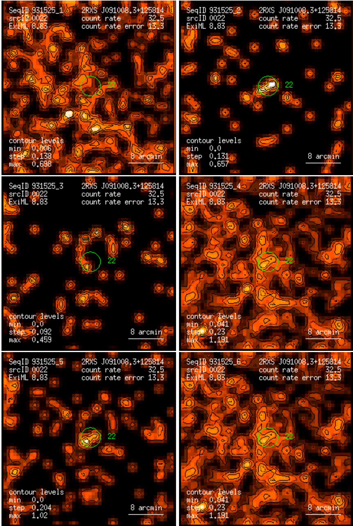
Figure 22: RASS 931525: detection 0022: band rate images, Gaussian filter: (1) PSPC channels 11 – 41, (2) 52 – 90, (3) 91 – 201, (4) 11 – 235, (5) 52 – 201, (6) 11 – 201. Broad band rates in counts/ks. Band rate contour levels in counts/ks/arcmin 2 .
