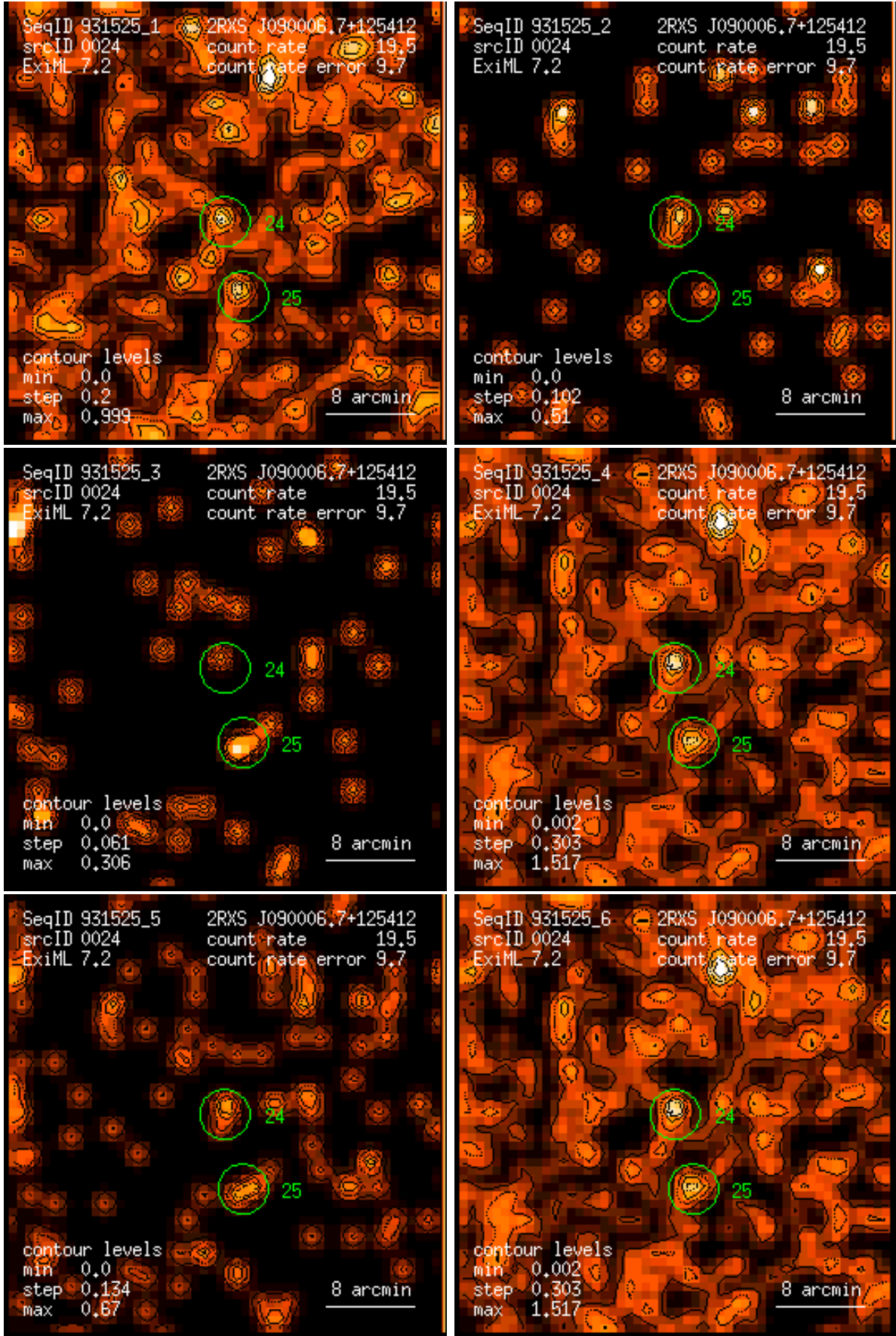
Figure 24: RASS 931525: detection 0024: band rate images, Gaussian filter: (1) PSPC channels 11 – 41, (2) 52 – 90, (3) 91 – 201, (4) 11 – 235, (5) 52 – 201, (6) 11 – 201. Broad band rates in counts/ks. Band rate contour levels in counts/ks/arcmin 2 .
