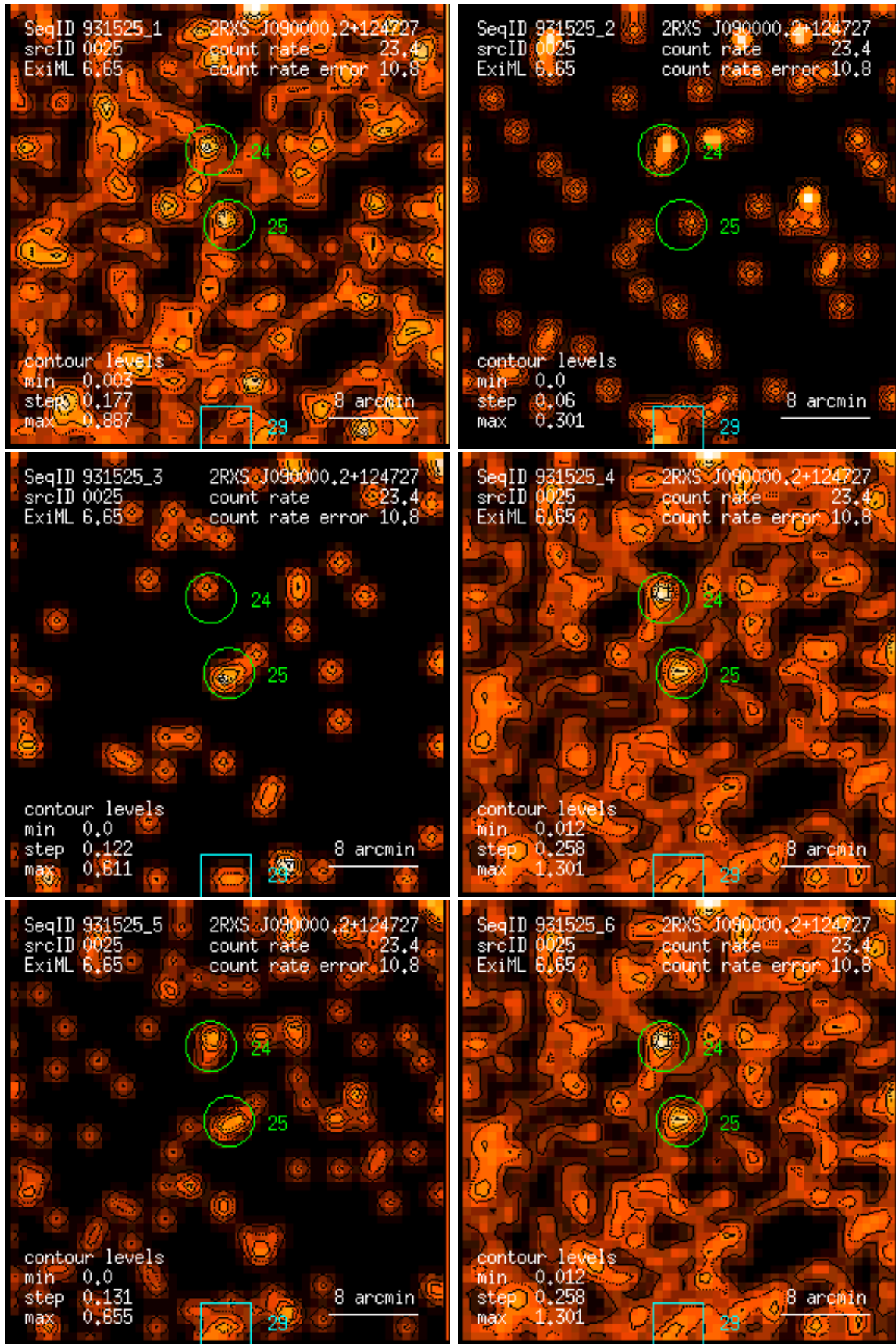
Figure 25: RASS 931525: detection 0025: band rate images, Gaussian filter: (1) PSPC channels 11 – 41, (2) 52 – 90, (3) 91 – 201, (4) 11 – 235, (5) 52 – 201, (6) 11 – 201. Broad band rates in counts/ks. Band rate contour levels in counts/ks/arcmin 2 .
