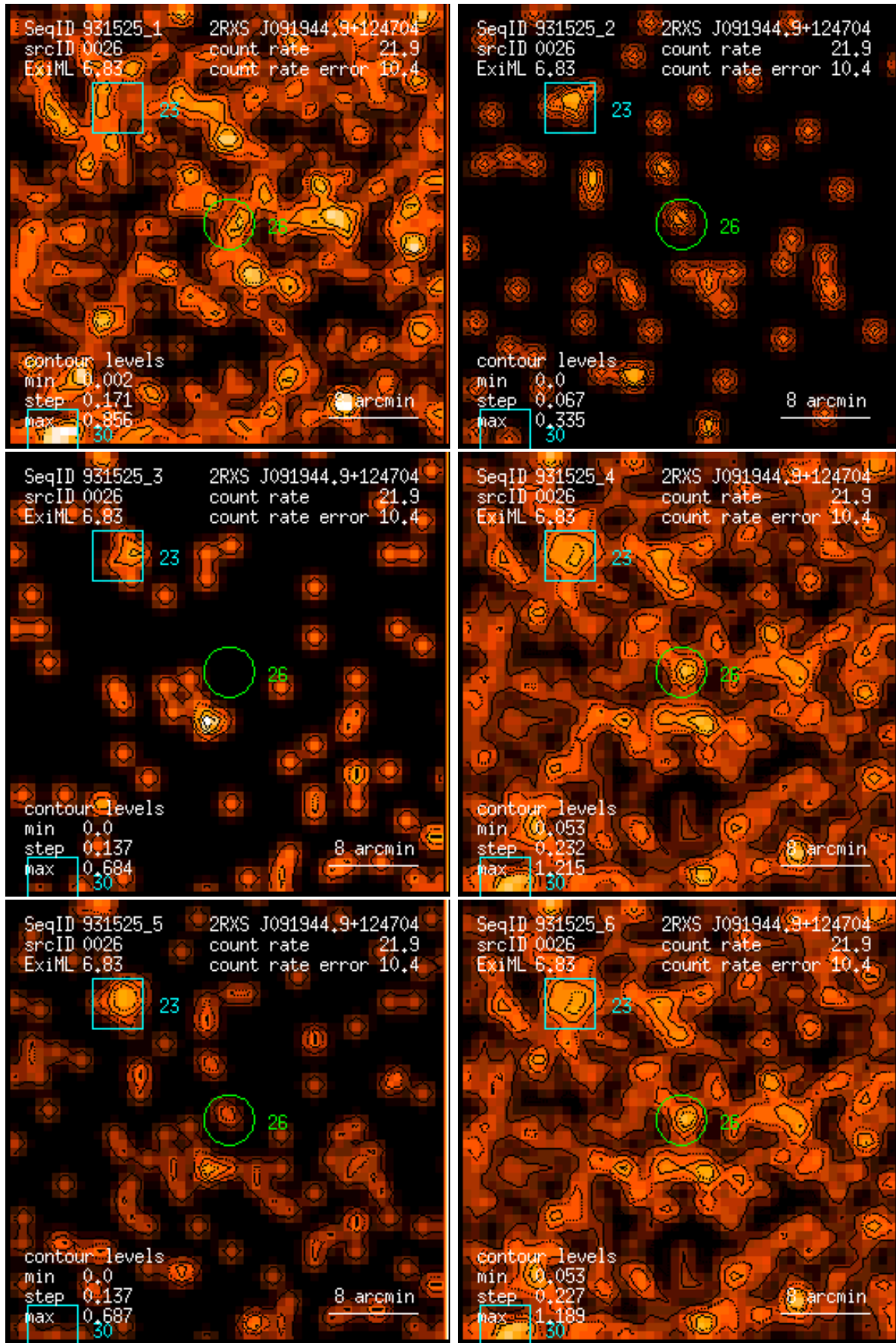
Figure 26: RASS 931525: detection 0026: band rate images, Gaussian filter: (1) PSPC channels 11 – 41, (2) 52 – 90, (3) 91 – 201, (4) 11 – 235, (5) 52 – 201, (6) 11 – 201. Broad band rates in counts/ks. Band rate contour levels in counts/ks/arcmin 2 .
