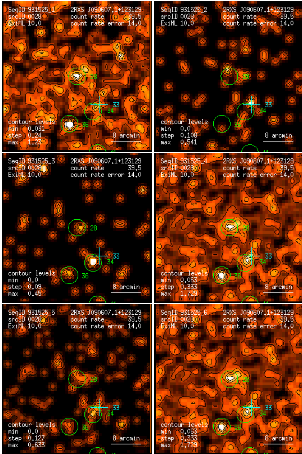
Figure 28: RASS 931525: detection 0028: band rate images, Gaussian filter: (1) PSPC channels 11 – 41, (2) 52 – 90, (3) 91 – 201, (4) 11 – 235, (5) 52 – 201, (6) 11 – 201. Broad band rates in counts/ks. Band rate contour levels in counts/ks/arcmin 2 .
