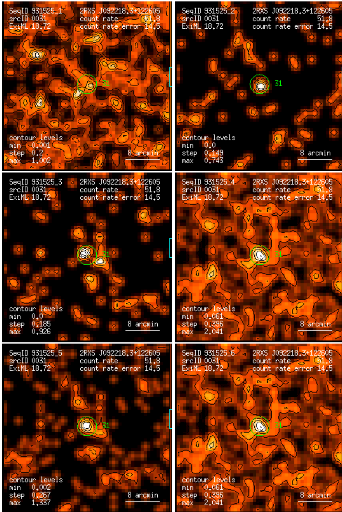
Figure 31: RASS 931525: detection 0031: band rate images, Gaussian filter: (1) PSPC channels 11 – 41, (2) 52 – 90, (3) 91 – 201, (4) 11 – 235, (5) 52 – 201, (6) 11 – 201. Broad band rates in counts/ks. Band rate contour levels in counts/ks/arcmin 2 .
