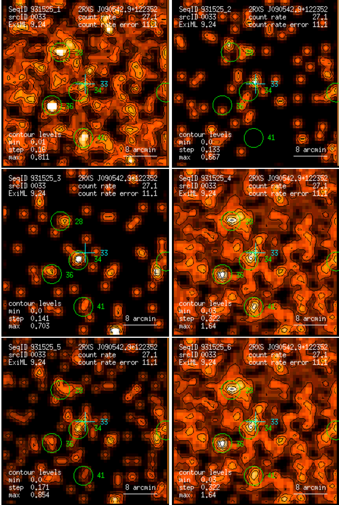
Figure 33: RASS 931525: detection 0033: band rate images, Gaussian filter: (1) PSPC channels 11 – 41, (2) 52 – 90, (3) 91 – 201, (4) 11 – 235, (5) 52 – 201, (6) 11 – 201. Broad band rates in counts/ks. Band rate contour levels in counts/ks/arcmin 2 .
