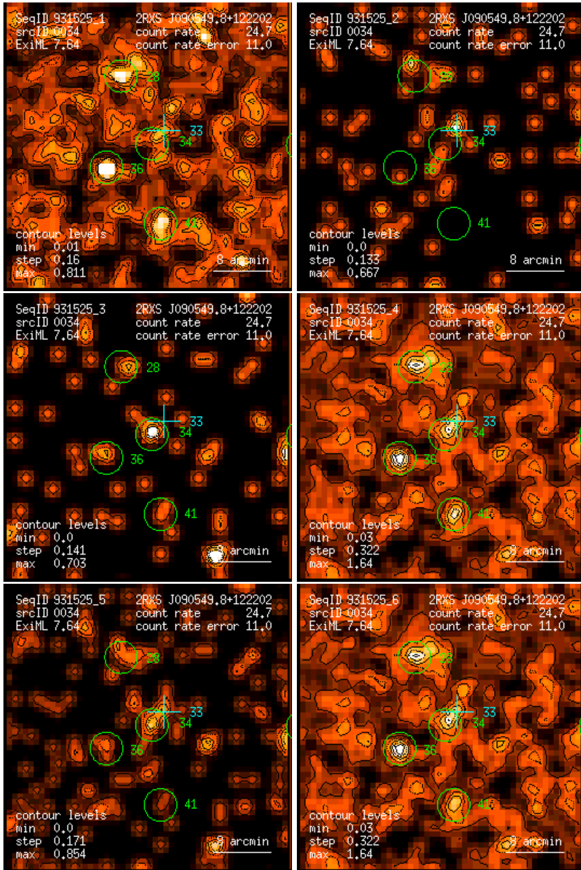
Figure 34: RASS 931525: detection 0034: band rate images, Gaussian filter: (1) PSPC channels 11 – 41, (2) 52 – 90, (3) 91 – 201, (4) 11 – 235, (5) 52 – 201, (6) 11 – 201. Broad band rates in counts/ks. Band rate contour levels in counts/ks/arcmin 2 .
