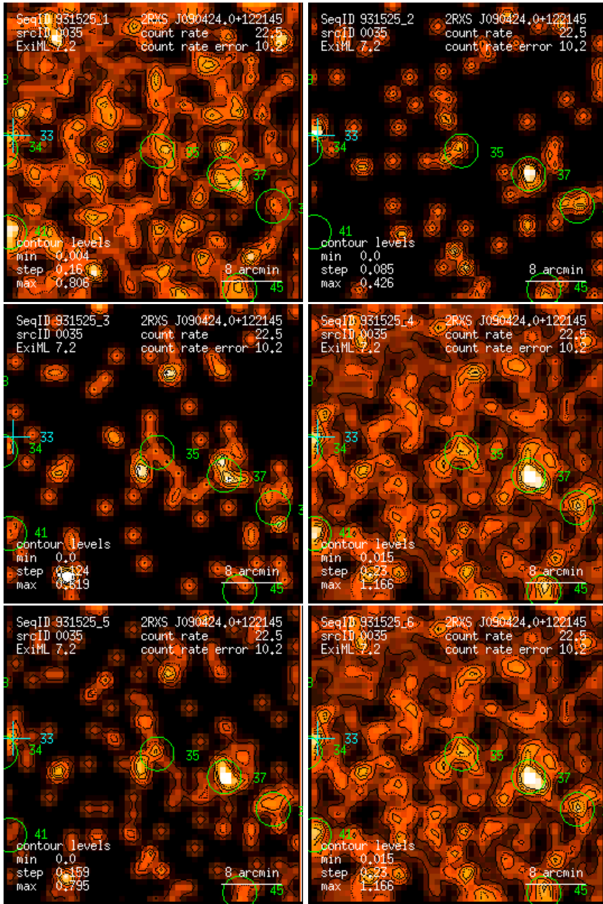
Figure 35: RASS 931525: detection 0035: band rate images, Gaussian filter: (1) PSPC channels 11 – 41, (2) 52 – 90, (3) 91 – 201, (4) 11 – 235, (5) 52 – 201, (6) 11 – 201. Broad band rates in counts/ks. Band rate contour levels in counts/ks/arcmin 2 .
