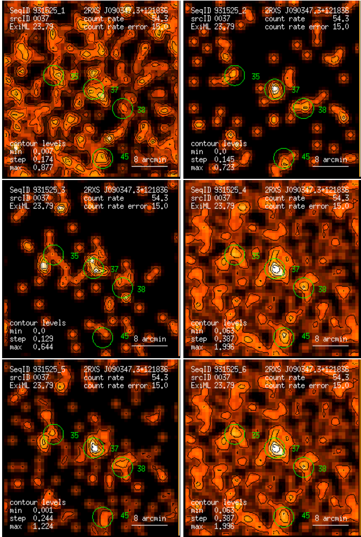
Figure 37: RASS 931525: detection 0037: band rate images, Gaussian filter: (1) PSPC channels 11 – 41, (2) 52 – 90, (3) 91 – 201, (4) 11 – 235, (5) 52 – 201, (6) 11 – 201. Broad band rates in counts/ks. Band rate contour levels in counts/ks/arcmin 2 .
