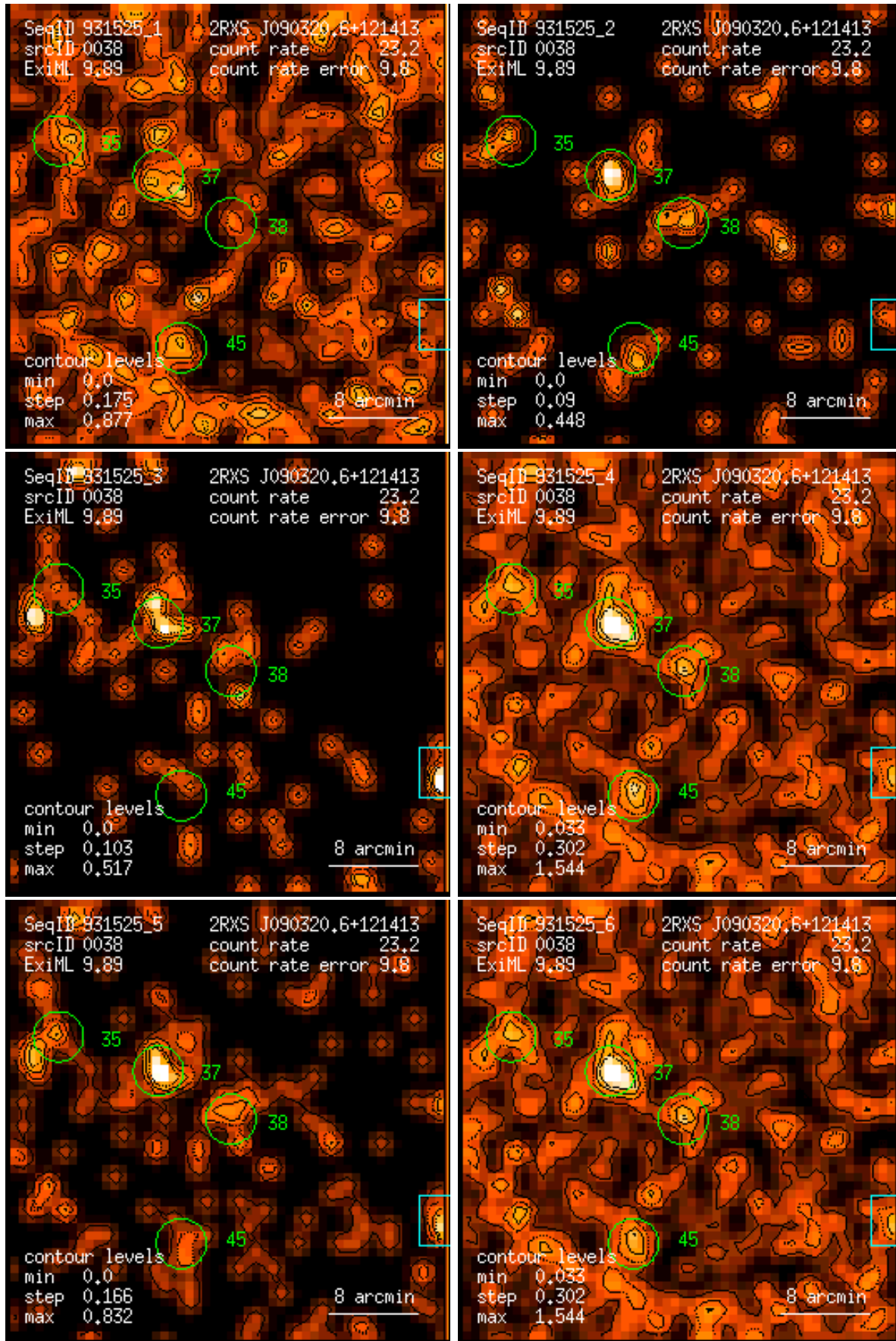
Figure 38: RASS 931525: detection 0038: band rate images, Gaussian filter: (1) PSPC channels 11 – 41, (2) 52 – 90, (3) 91 – 201, (4) 11 – 235, (5) 52 – 201, (6) 11 – 201. Broad band rates in counts/ks. Band rate contour levels in counts/ks/arcmin 2 .
