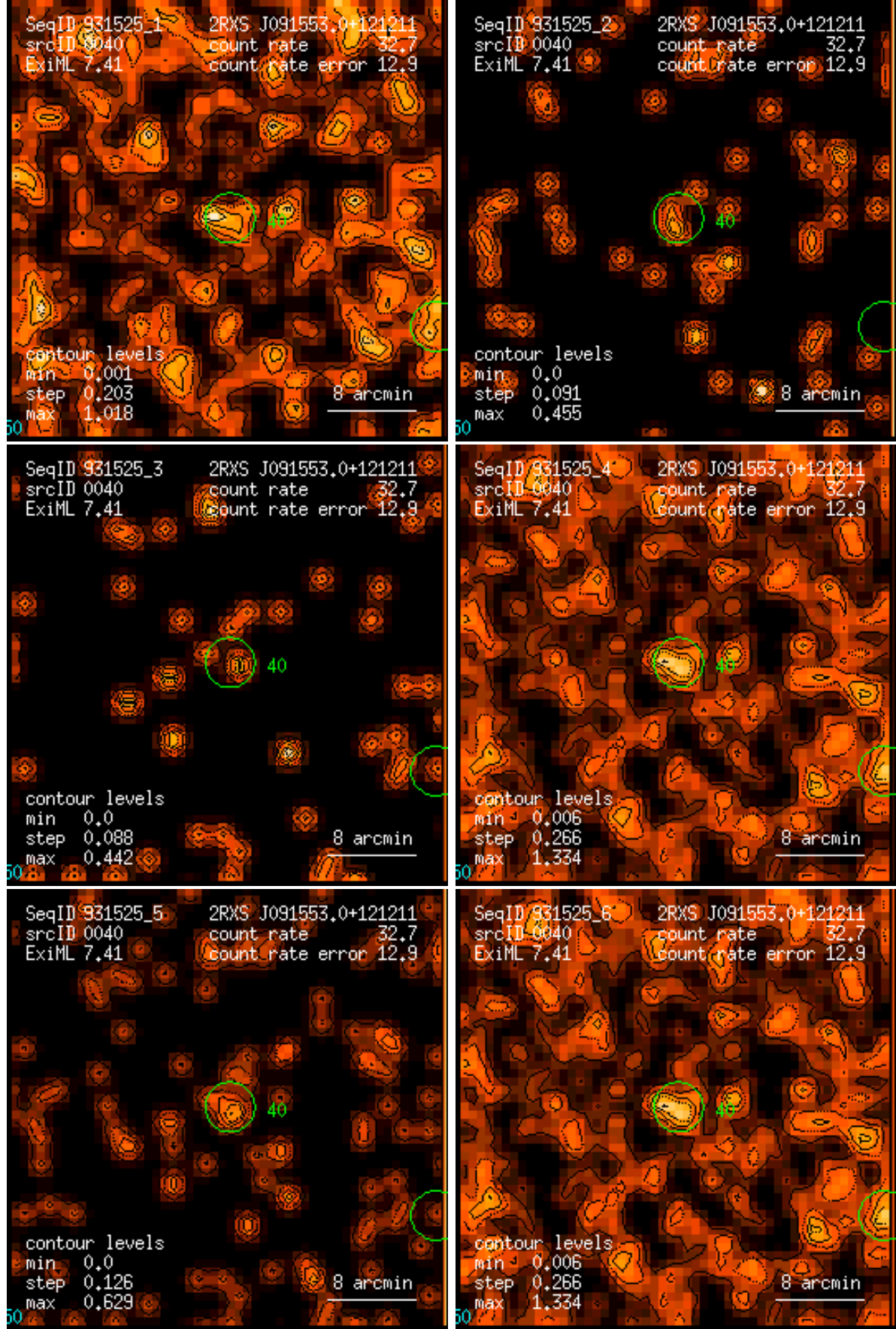
Figure 40: RASS 931525: detection 0040: band rate images, Gaussian filter: (1) PSPC channels 11 – 41, (2) 52 – 90, (3) 91 – 201, (4) 11 – 235, (5) 52 – 201, (6) 11 – 201. Broad band rates in counts/ks. Band rate contour levels in counts/ks/arcmin 2 .
