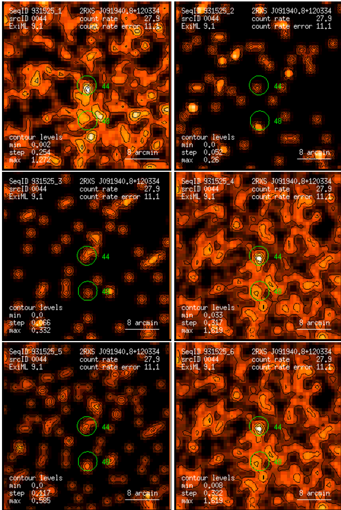
Figure 44: RASS 931525: detection 0044: band rate images, Gaussian filter: (1) PSPC channels 11 – 41, (2) 52 – 90, (3) 91 – 201, (4) 11 – 235, (5) 52 – 201, (6) 11 – 201. Broad band rates in counts/ks. Band rate contour levels in counts/ks/arcmin 2 .
