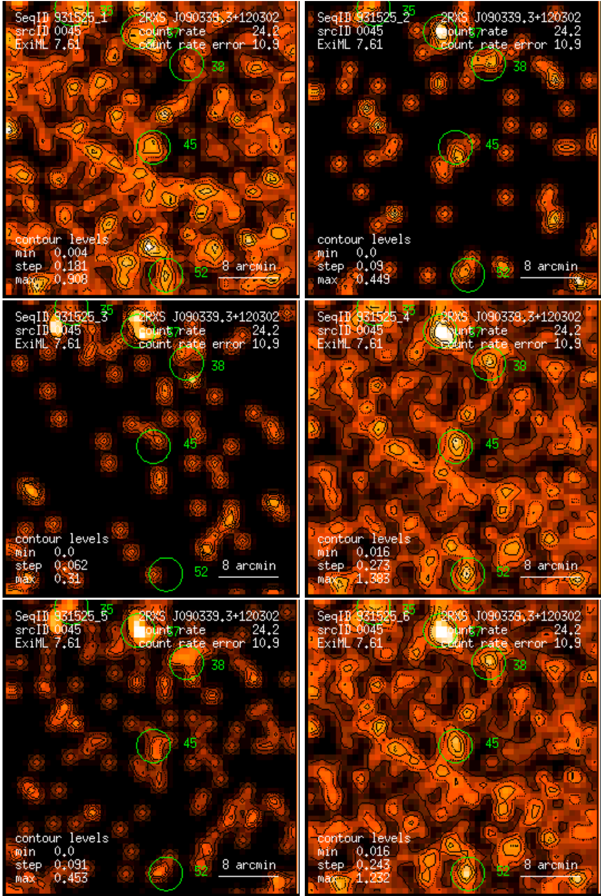
Figure 45: RASS 931525: detection 0045: band rate images, Gaussian filter: (1) PSPC channels 11 – 41, (2) 52 – 90, (3) 91 – 201, (4) 11 – 235, (5) 52 – 201, (6) 11 – 201. Broad band rates in counts/ks. Band rate contour levels in counts/ks/arcmin 2 .
