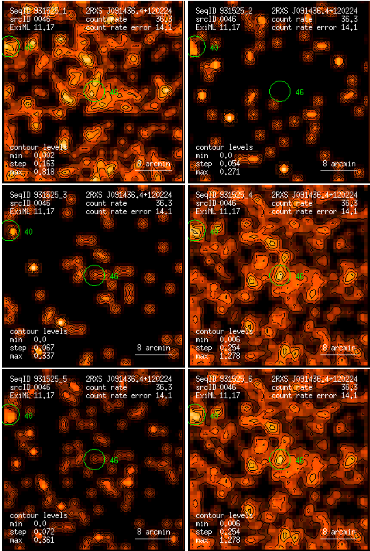
Figure 46: RASS 931525: detection 0046: band rate images, Gaussian filter: (1) PSPC channels 11 – 41, (2) 52 – 90, (3) 91 – 201, (4) 11 – 235, (5) 52 – 201, (6) 11 – 201. Broad band rates in counts/ks. Band rate contour levels in counts/ks/arcmin 2 .
