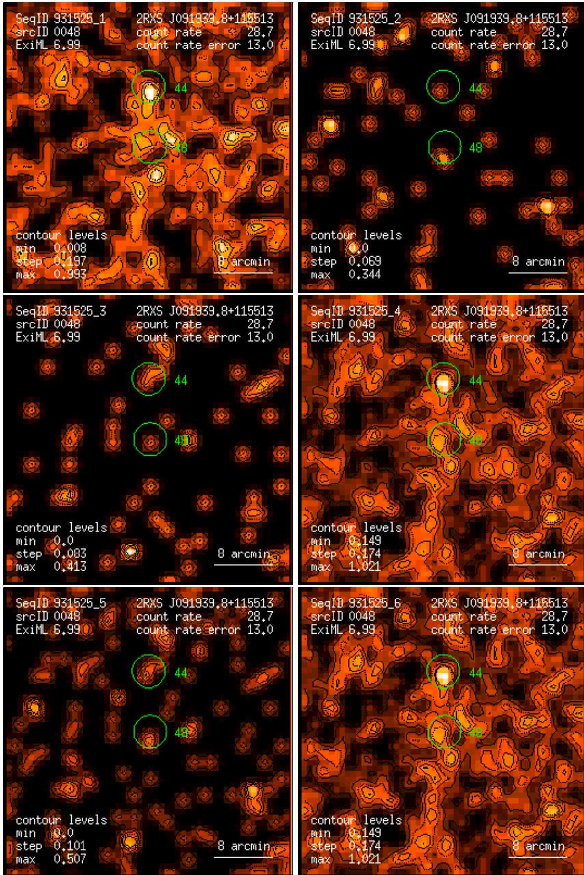
Figure 48: RASS 931525: detection 0048: band rate images, Gaussian filter: (1) PSPC channels 11 – 41, (2) 52 – 90, (3) 91 – 201, (4) 11 – 235, (5) 52 – 201, (6) 11 – 201. Broad band rates in counts/ks. Band rate contour levels in counts/ks/arcmin 2 .
