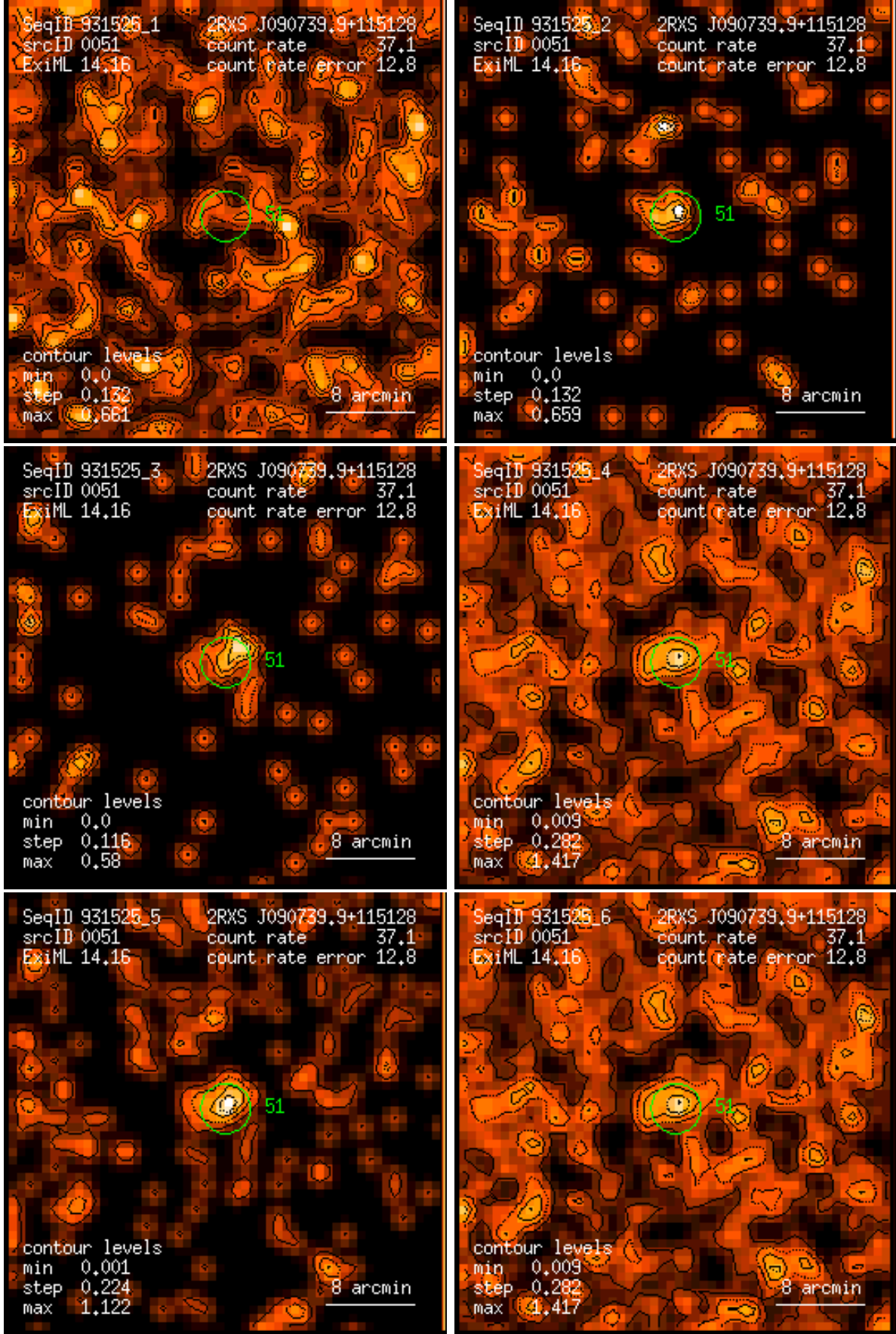
Figure 51: RASS 931525: detection 0051: band rate images, Gaussian filter: (1) PSPC channels 11 – 41, (2) 52 – 90, (3) 91 – 201, (4) 11 – 235, (5) 52 – 201, (6) 11 – 201. Broad band rates in counts/ks. Band rate contour levels in counts/ks/arcmin 2 .
