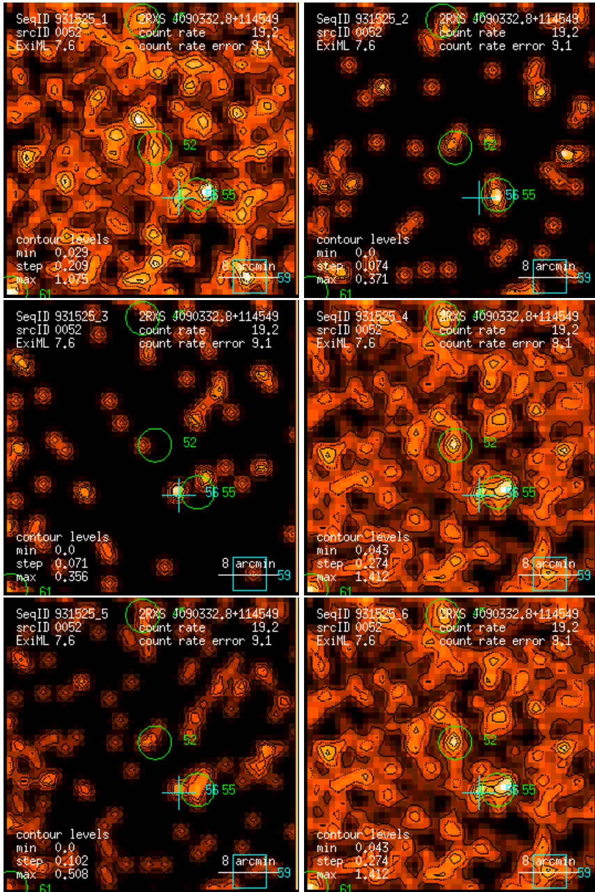
Figure 52: RASS 931525: detection 0052: band rate images, Gaussian filter: (1) PSPC channels 11 – 41, (2) 52 – 90, (3) 91 – 201, (4) 11 – 235, (5) 52 – 201, (6) 11 – 201. Broad band rates in counts/ks. Band rate contour levels in counts/ks/arcmin 2 .
