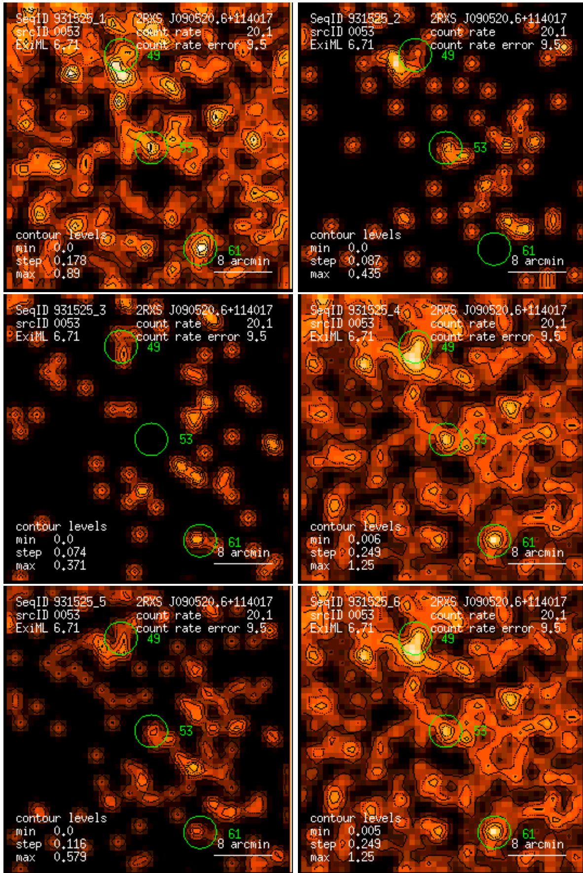
Figure 53: RASS 931525: detection 0053: band rate images, Gaussian filter: (1) PSPC channels 11 – 41, (2) 52 – 90, (3) 91 – 201, (4) 11 – 235, (5) 52 – 201, (6) 11 – 201. Broad band rates in counts/ks. Band rate contour levels in counts/ks/arcmin 2 .
