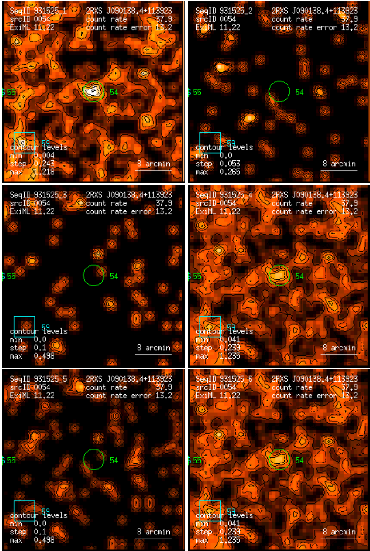
Figure 54: RASS 931525: detection 0054: band rate images, Gaussian filter: (1) PSPC channels 11 – 41, (2) 52 – 90, (3) 91 – 201, (4) 11 – 235, (5) 52 – 201, (6) 11 – 201. Broad band rates in counts/ks. Band rate contour levels in counts/ks/arcmin 2 .
