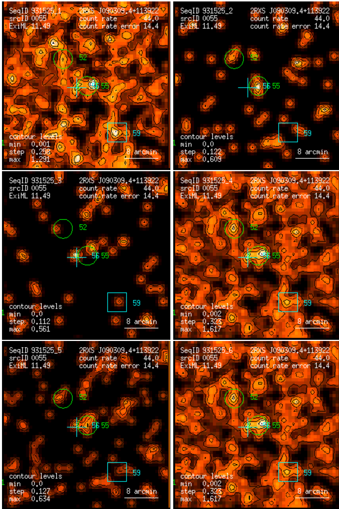
Figure 55: RASS 931525: detection 0055: band rate images, Gaussian filter: (1) PSPC channels 11 – 41, (2) 52 – 90, (3) 91 – 201, (4) 11 – 235, (5) 52 – 201, (6) 11 – 201. Broad band rates in counts/ks. Band rate contour levels in counts/ks/arcmin 2 .
