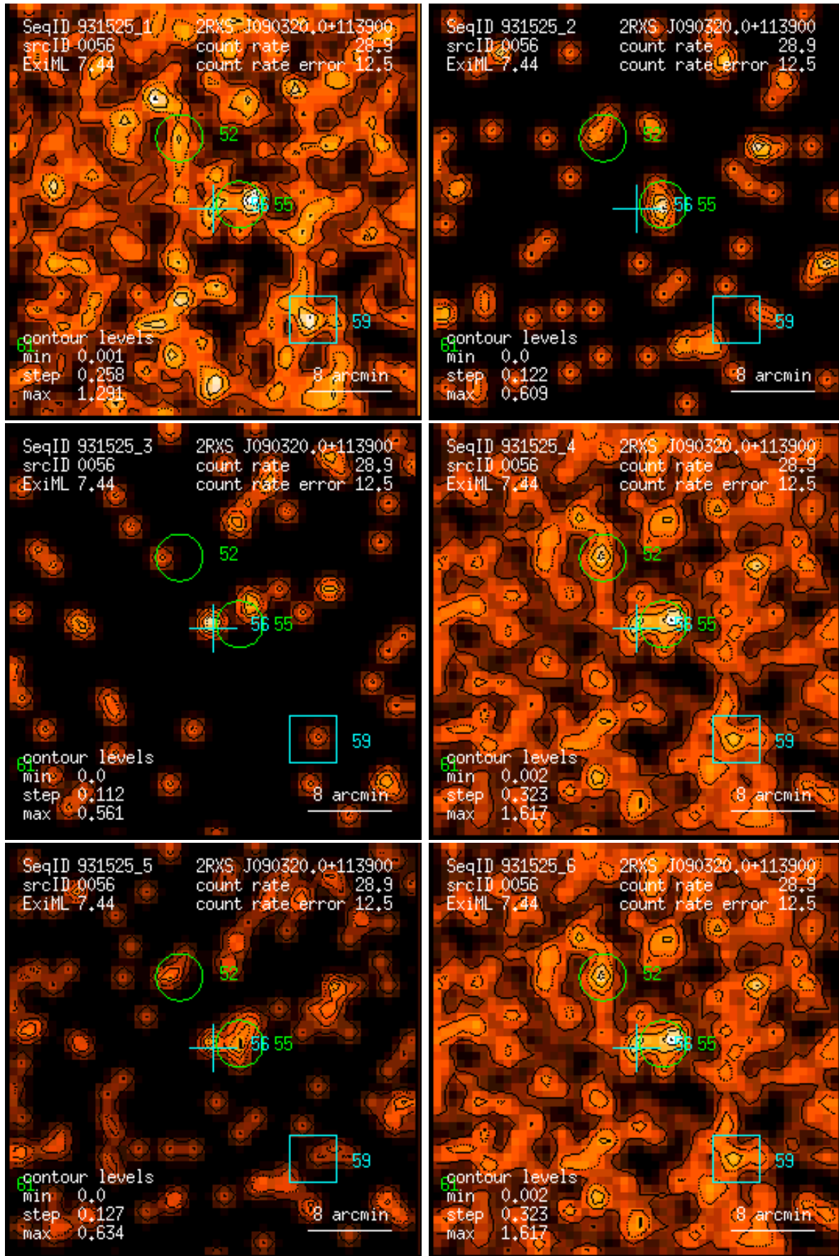
Figure 56: RASS 931525: detection 0056: band rate images, Gaussian filter: (1) PSPC channels 11 – 41, (2) 52 – 90, (3) 91 – 201, (4) 11 – 235, (5) 52 – 201, (6) 11 – 201. Broad band rates in counts/ks. Band rate contour levels in counts/ks/arcmin 2 .
