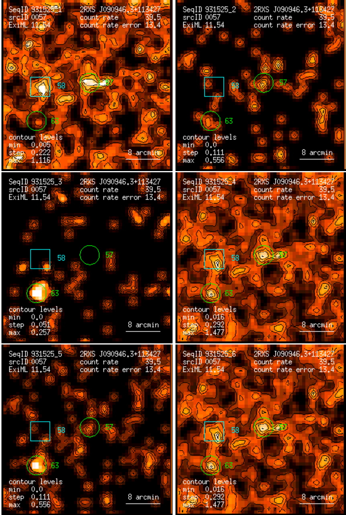
Figure 57: RASS 931525: detection 0057: band rate images, Gaussian filter: (1) PSPC channels 11 – 41, (2) 52 – 90, (3) 91 – 201, (4) 11 – 235, (5) 52 – 201, (6) 11 – 201. Broad band rates in counts/ks. Band rate contour levels in counts/ks/arcmin 2 .
